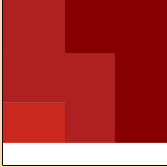
\Delta\sigma/\sigma vs. E for ^{160}\text{Yb}(n,\text{el.})
