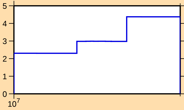
\Delta\sigma/\sigma vs. E for ^{160}\text{Yb}(n,\text{tot.})
