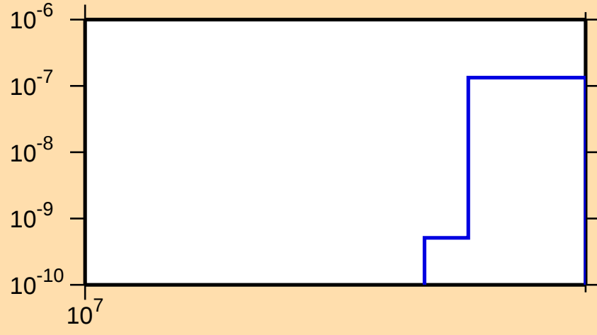
\sigma vs. E for ^{160}\text{Yb}(n,\text{nd})
