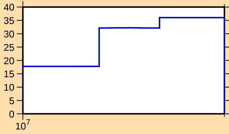
\Delta\sigma/\sigma vs. E for ^{160}\text{Yb}(n,\text{inel.})
