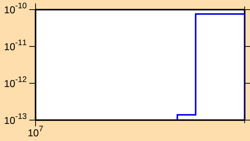
\sigma vs. E for ^{160}\text{Yb}(n,\text{pt})
