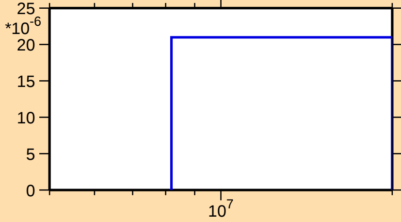
\sigma vs. E for ^{160}\text{Yb}(n,t)
