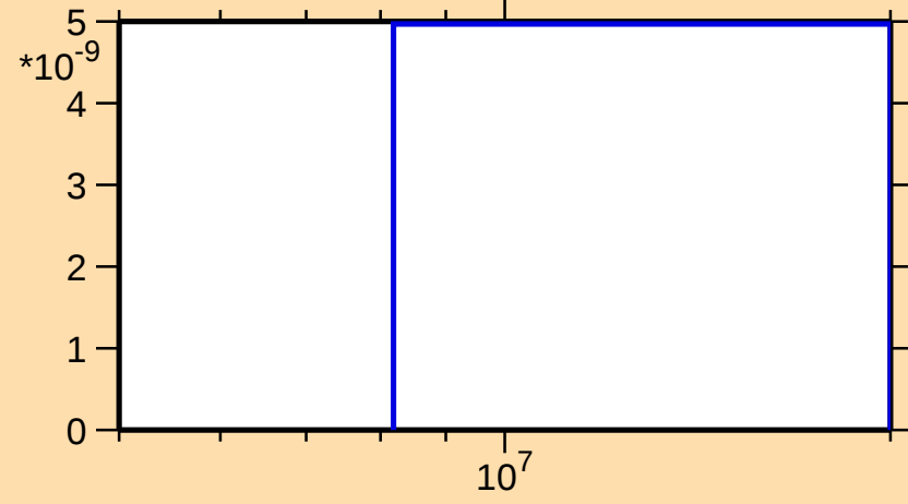
\sigma vs. E for ^{160}\text{Yb}(n,\text{pd})
