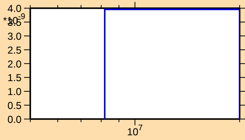
\sigma vs. E for ^{160}\text{Yb} (mt 45)
