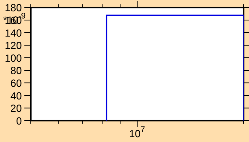
\sigma vs. E for ^{160}\text{Yb}(n,\text{He}3)
