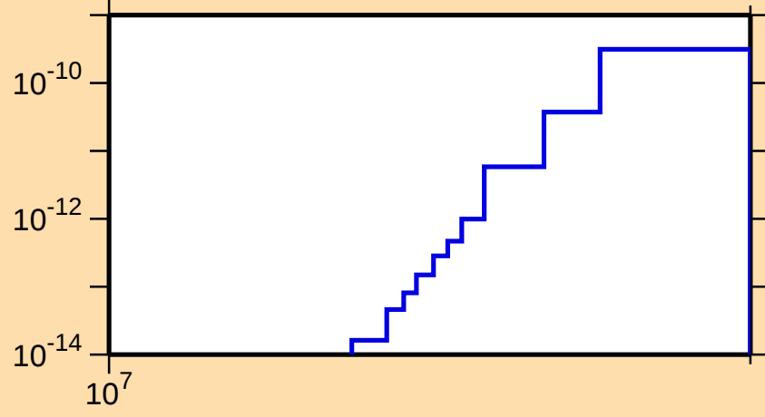
\sigma vs. E for ^{161}\text{Yb}(\text{mt117})
