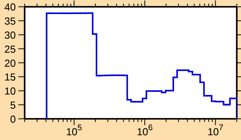
\Delta\sigma/\sigma vs. E for ^{161}\text{Yb}(n,\text{el.})
