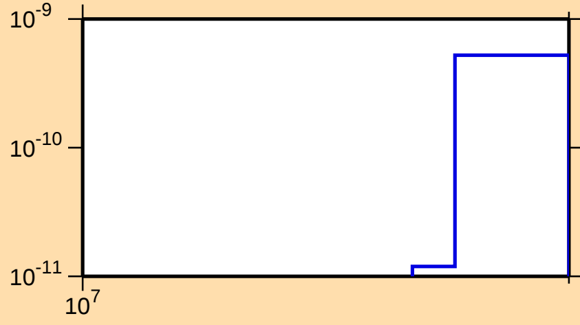
\sigma vs. E for ^{161}\text{Yb} (mt 34)
