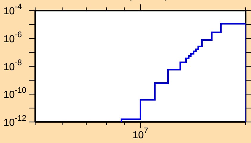
\sigma vs. E for ^{161}\text{Yb}(n,\text{He3})
