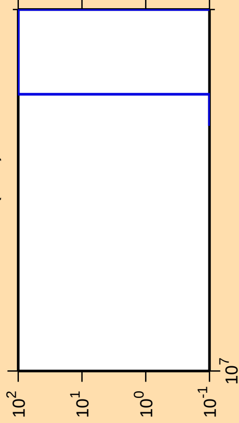
\Delta\sigma/\sigma vs. E for ^{161}\text{Yb}(n,nt)
