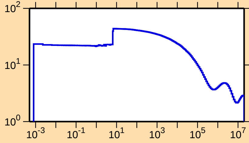
\sigma vs. E for ^{161}\text{Yb}(n,\text{el.})
