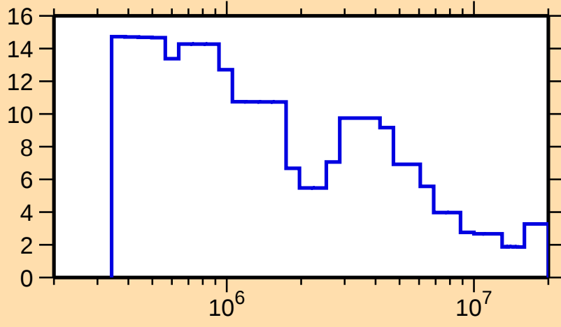
\Delta\sigma/\sigma vs. E for ^{161}\text{Yb}(n,\text{tot.})
