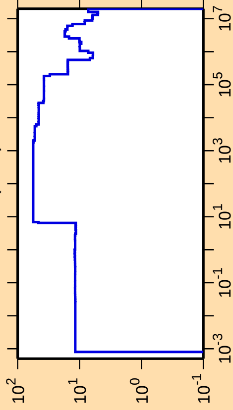
\Delta\sigma/\sigma vs. E for ^{161}\text{Yb}(n,\text{el.})
