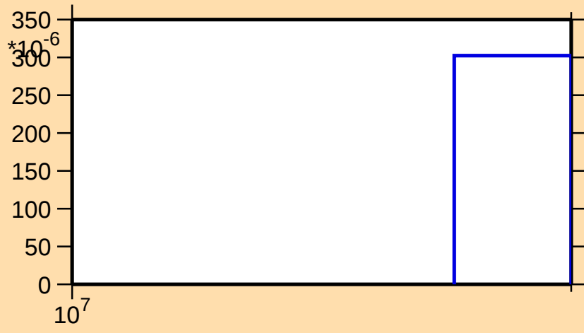
\sigma vs. E for ^{161}\text{Yb}(n,3n)
