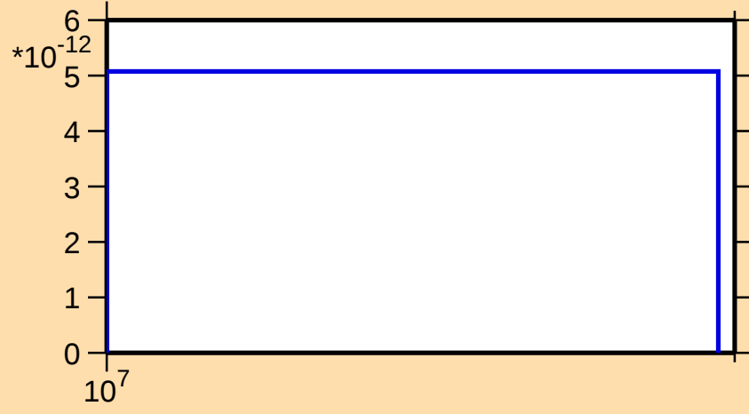
\sigma vs. E for ^{161}\text{Yb} (mt 34)
