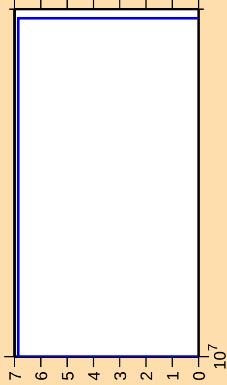
\Delta\sigma/\sigma vs. E for ^{161}\text{Yb}(n,nt)
