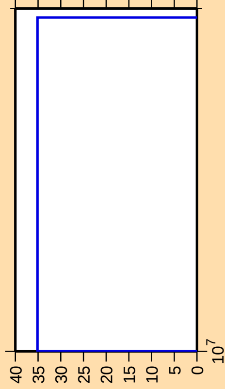
\Delta\sigma/\sigma vs. E for ^{161}\text{Yb} (mt 34)
