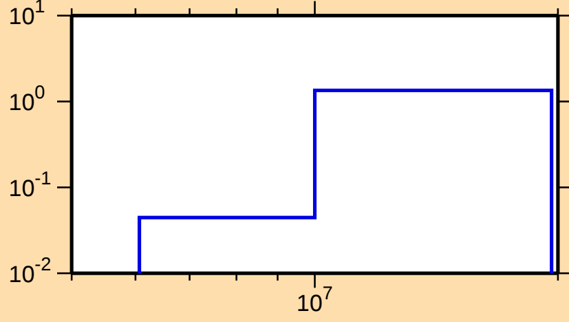
\sigma vs. E for ^{161}\text{Yb}(n,2n)
