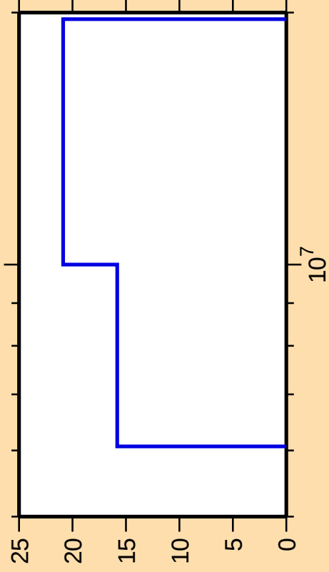
\Delta\sigma/\sigma vs. E for ^{161}\text{Yb}(n,n\text{cont.})
