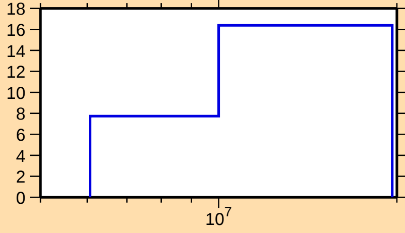
\Delta\sigma/\sigma vs. E for ^{161}\text{Yb}(n,\text{inel.})
