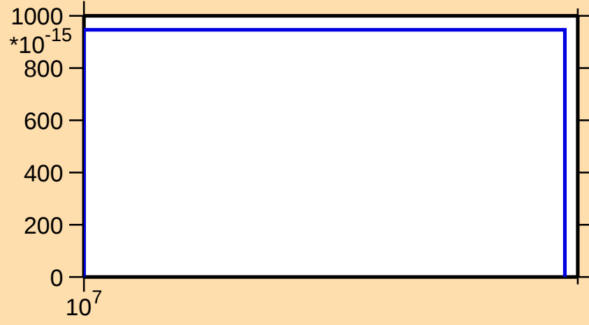
\sigma vs. E for ^{161}\text{Yb}(n,nt)
