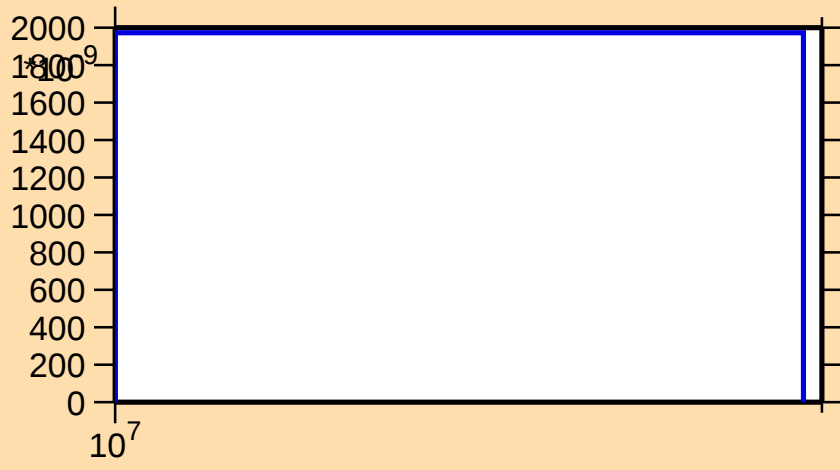
\sigma vs. E for ^{161}\text{Yb}(n,3n)
