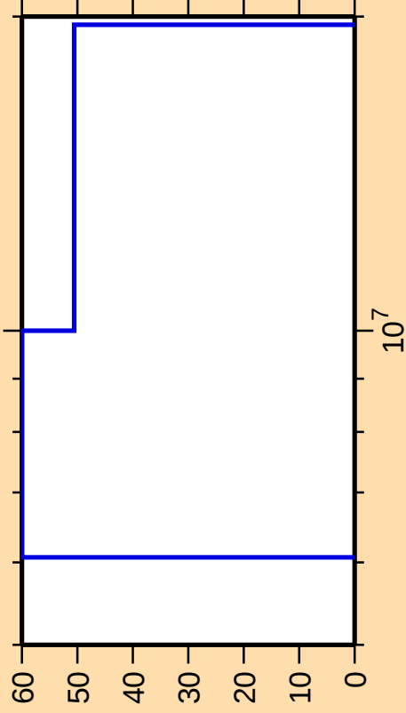
\Delta\sigma/\sigma vs. E for ^{161}\text{Yb}(n,n_1)
