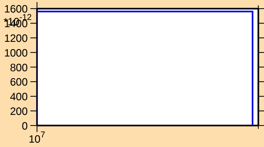
\sigma vs. E for ^{161}\text{Yb}(n,\text{pd})
