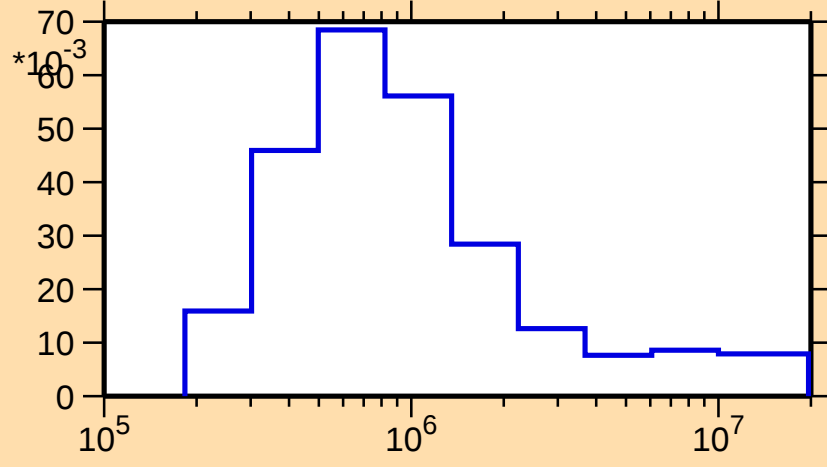
\sigma vs. E for ^{161}\text{Yb}(n,n_3)
