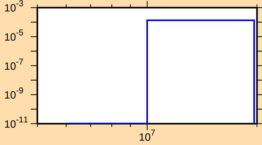
\sigma vs. E for ^{161}\text{Yb}(n,t)
