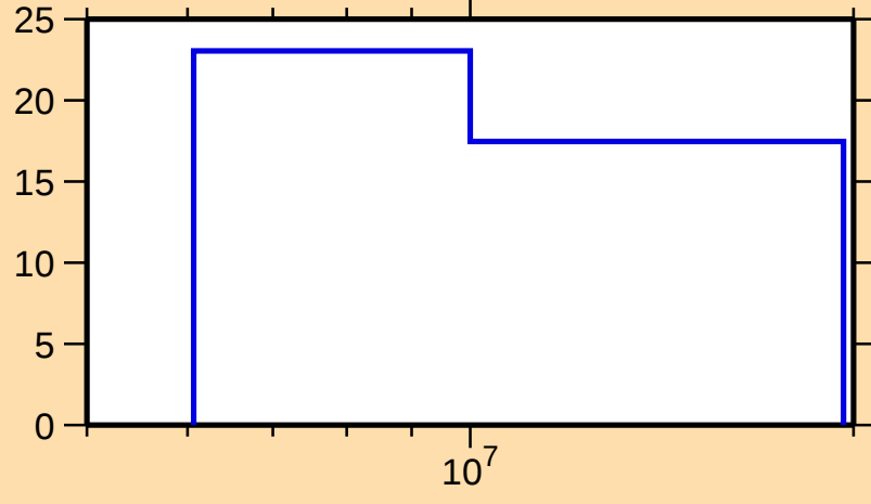
\Delta\sigma/\sigma vs. E for ^{161}\text{Yb}(n,2n)
