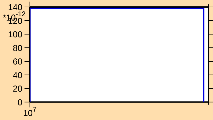
\sigma vs. E for ^{161}\text{Yb}(n,\text{pt})
