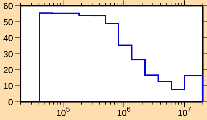
\Delta\sigma/\sigma vs. E for ^{161}\text{Yb}(n,\text{inel.})
