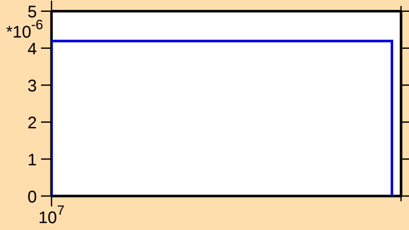
\sigma vs. E for ^{161}\text{Yb}(n,2np)
