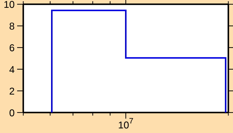
\Delta\sigma/\sigma vs. E for ^{161}\text{Yb}(n,\text{el.})
