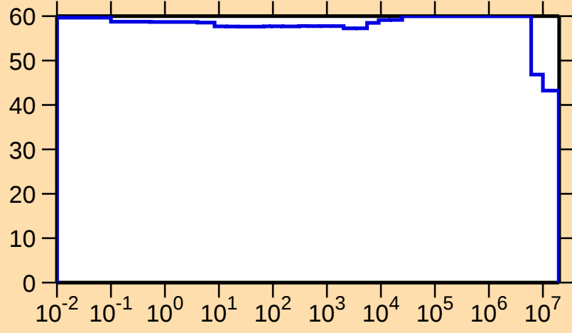
\Delta\sigma/\sigma vs. E for ^{161}\text{Yb}(n,p)
