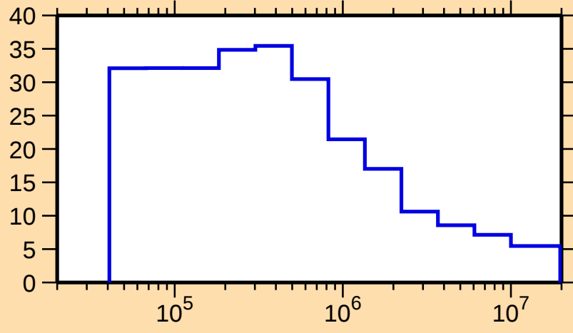
\Delta\sigma/\sigma vs. E for ^{161}\text{Yb}(n,\text{nonel.})
