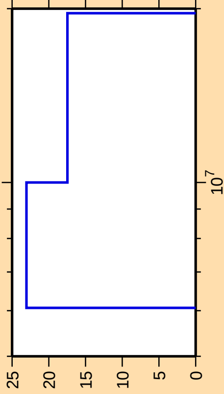
\Delta\sigma/\sigma vs. E for ^{161}\text{Yb}(n,2n)
