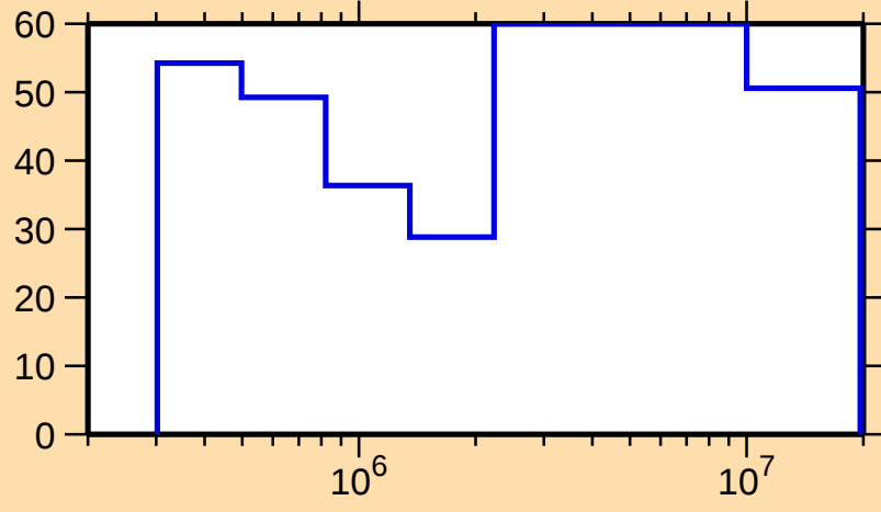
\Delta\sigma/\sigma vs. E for ^{161}\text{Yb}(n,n_1)
