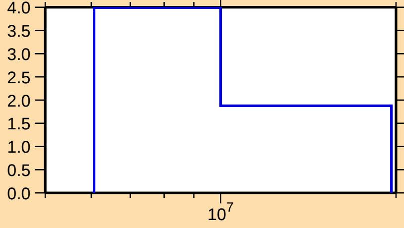
\Delta\sigma/\sigma vs. E for ^{161}\text{Yb}(n,\text{tot.})
