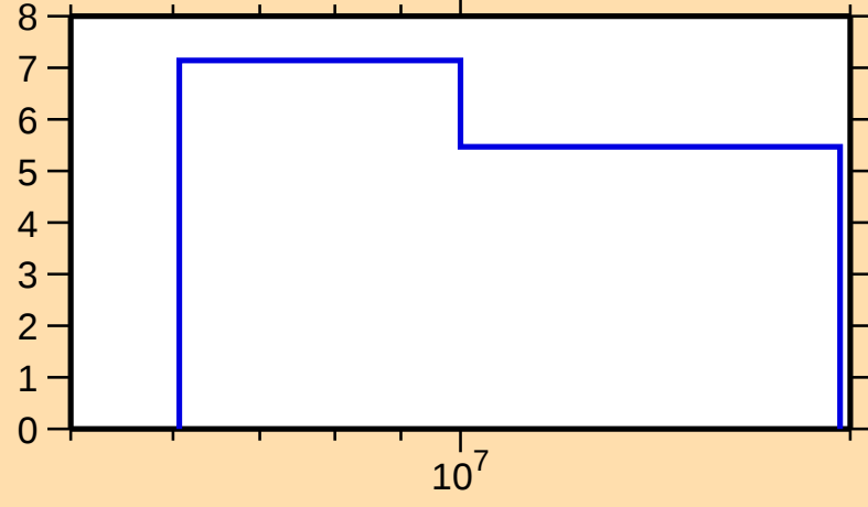
\Delta\sigma/\sigma vs. E for ^{161}\text{Yb}(n,\text{nonel.})
