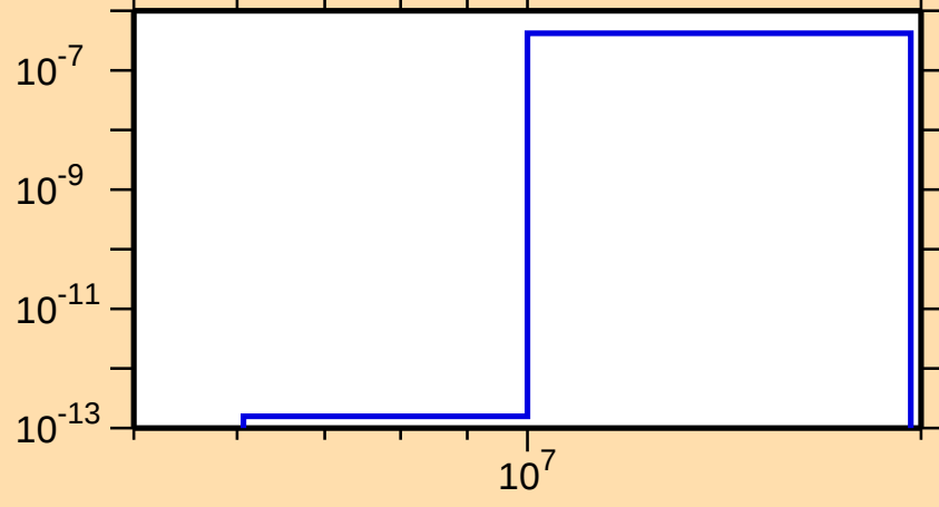
\sigma vs. E for ^{161}\text{Yb}(n,\text{He3})
