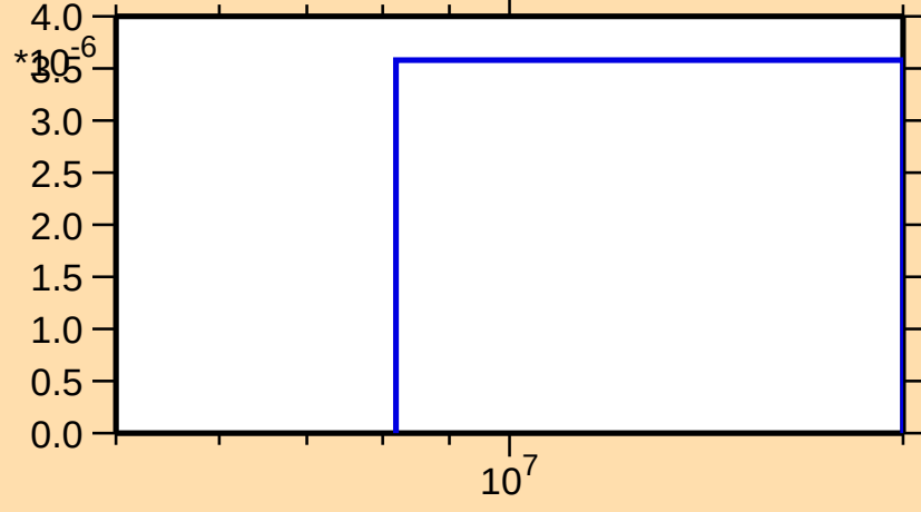
\sigma vs. E for ^{161}\text{Yb}(n,2np)
