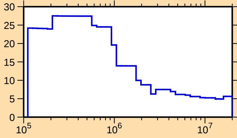
\Delta\sigma/\sigma vs. E for ^{164}\text{Yb}(n,\text{nonel.})
