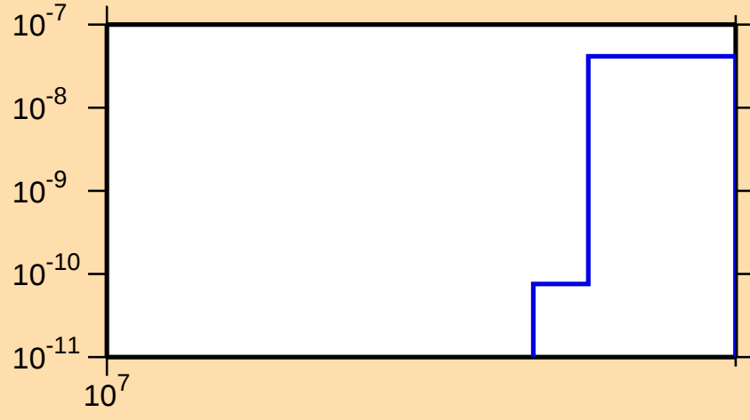
\sigma vs. E for ^{164}\text{Yb}(n,\text{nd})
