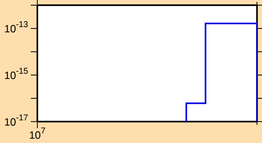
\sigma vs. E for ^{164}\text{Yb} (mt 34)
