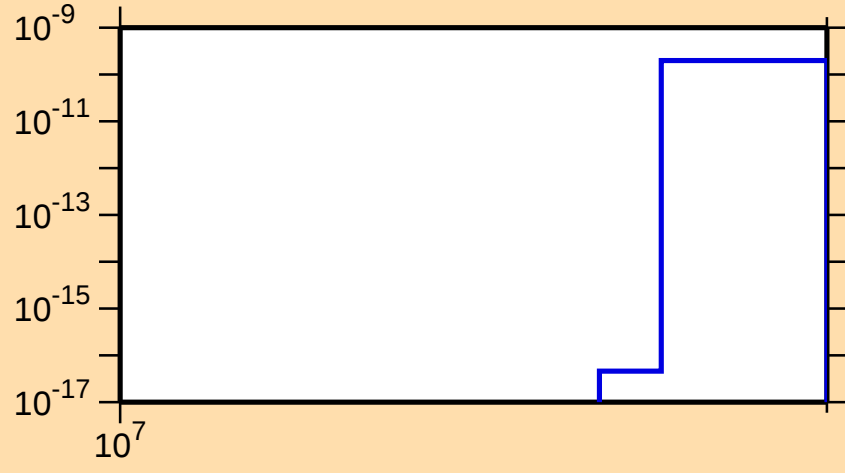
\sigma vs. E for ^{164}\text{Yb}(n,nt)
