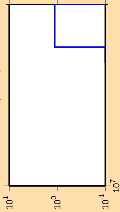
\Delta\sigma/\sigma vs. E for ^{164}\text{Yb} (mt 34)
