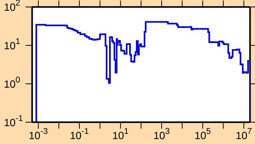
\Delta\sigma/\sigma vs. E for ^{164}\text{Yb}(n,\text{tot.})
