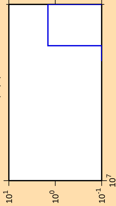
\Delta\sigma/\sigma vs. E for ^{164}\text{Yb}(n,\text{pt})
