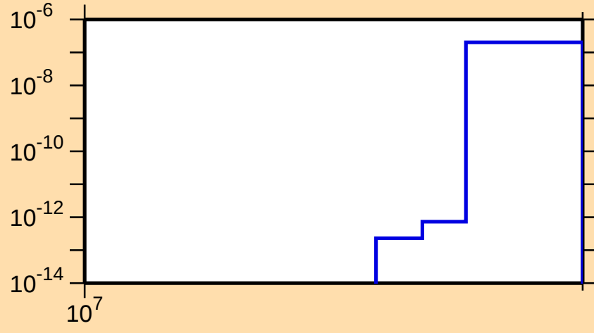
\sigma vs. E for ^{164}\text{Yb}(n,2np)
