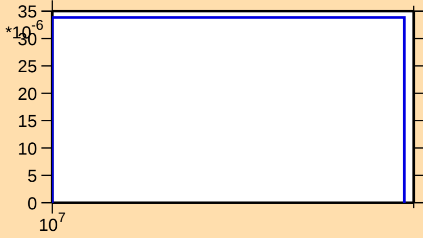
\sigma vs. E for ^{164}\text{Yb}(n,3n)
