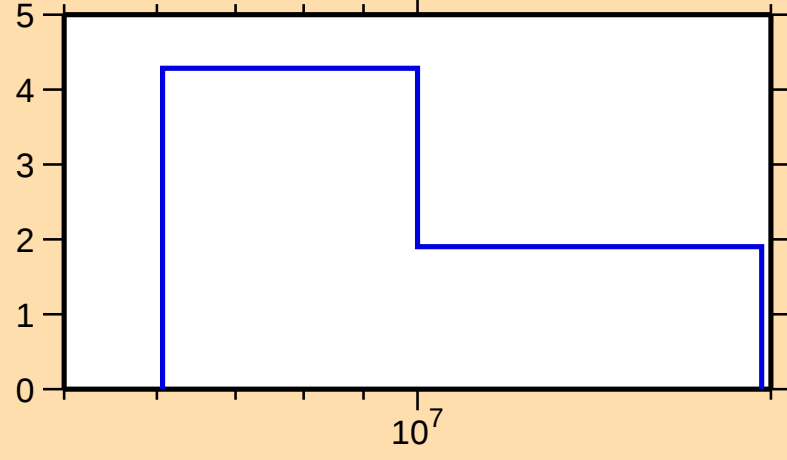
\Delta\sigma/\sigma vs. E for ^{164}\text{Yb}(n,\text{tot.})
