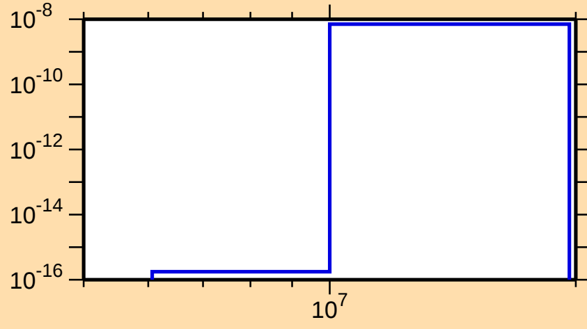
\sigma vs. E for ^{164}\text{Yb}(n,\text{He}3)
