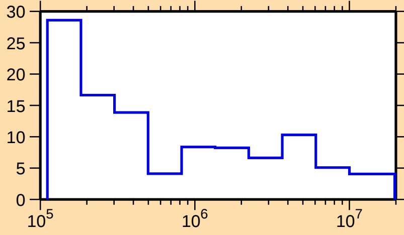
\Delta\sigma/\sigma vs. E for ^{164}\text{Yb}(n,\text{el.})
