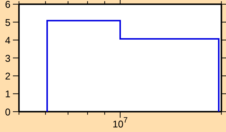
\Delta\sigma/\sigma vs. E for ^{164}\text{Yb}(n,\text{el.})
