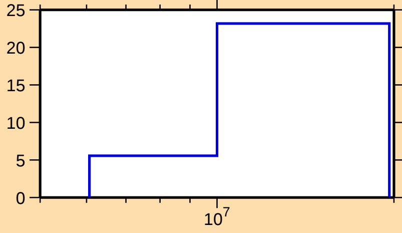
\Delta\sigma/\sigma vs. E for ^{164}\text{Yb}(n,\text{inel.})
