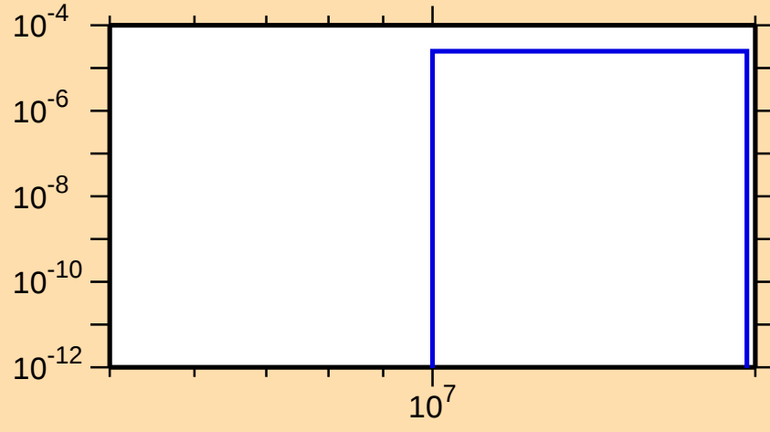
\sigma vs. E for ^{164}\text{Yb}(n,t)
