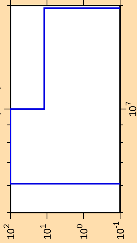
\Delta\sigma/\sigma vs. E for ^{164}\text{Yb}(n,2n)
