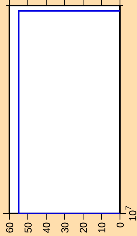
\Delta\sigma/\sigma vs. E for ^{164}\text{Yb}(n,\text{pd})
