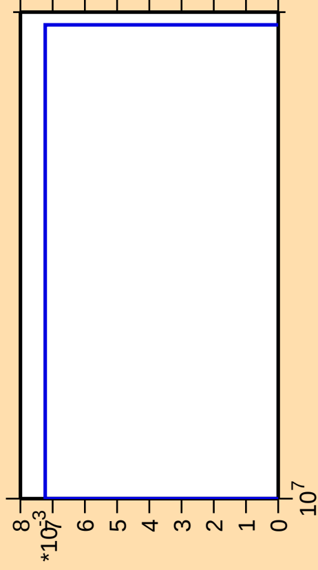
\Delta\sigma/\sigma vs. E for ^{164}\text{Yb}(\text{mt } 34)
