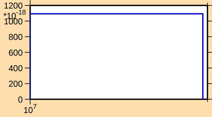
\sigma vs. E for ^{164}\text{Yb}(\text{mt } 34)
