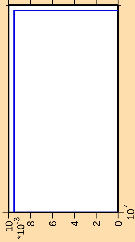
\Delta\sigma/\sigma vs. E for ^{164}\text{Yb}(n,\text{pt})
