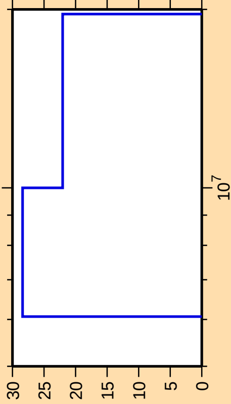
\Delta\sigma/\sigma vs. E for ^{164}\text{Yb}(n,n_1)
