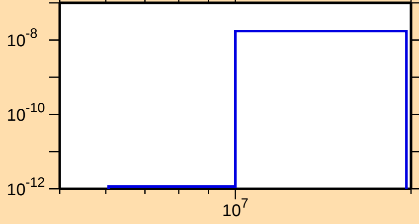
\sigma vs. E for ^{164}\text{Yb}(n,p\alpha)
