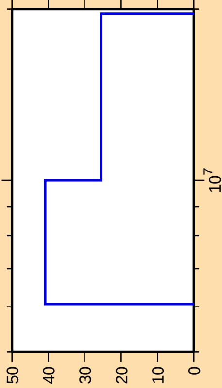
\Delta\sigma/\sigma vs. E for ^{164}\text{Yb}(n,p)
