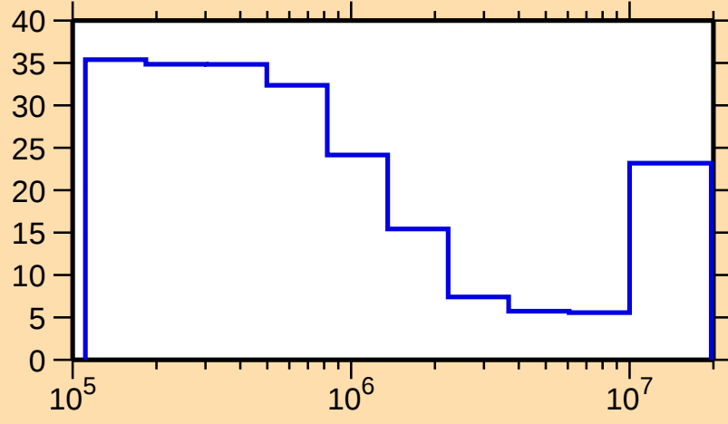
\Delta\sigma/\sigma vs. E for ^{164}\text{Yb}(n,\text{inel.})
