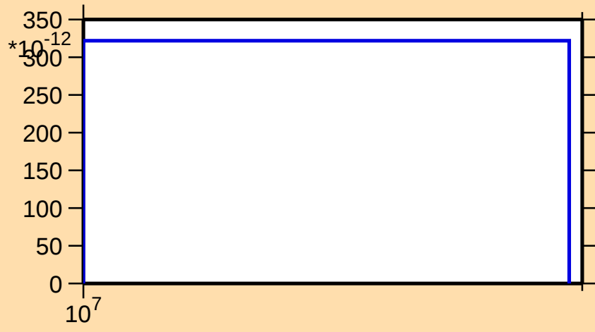
\sigma vs. E for ^{164}\text{Yb}(n,\text{nd})
