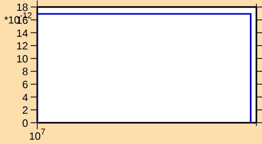
\sigma vs. E for ^{164}\text{Yb}(n,\text{pd})
