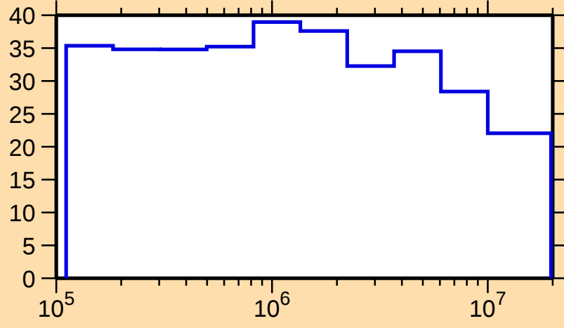
\Delta\sigma/\sigma vs. E for ^{164}\text{Yb}(n,n_1)
