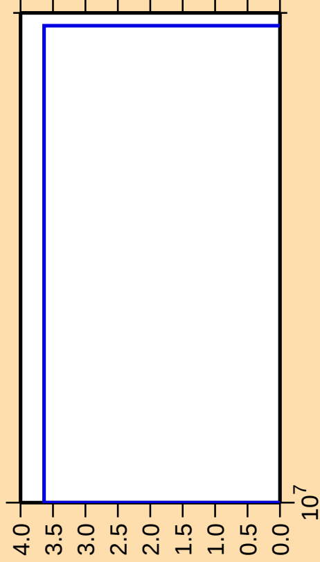
\Delta\sigma/\sigma vs. E for ^{164}\text{Yb}(n,nt)
