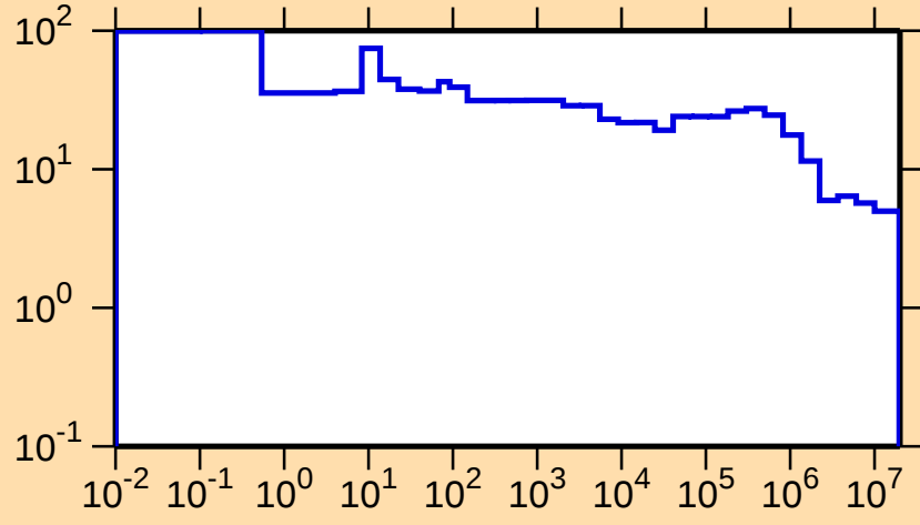
\Delta\sigma/\sigma vs. E for ^{164}\text{Yb}(n,\text{nonel.})
