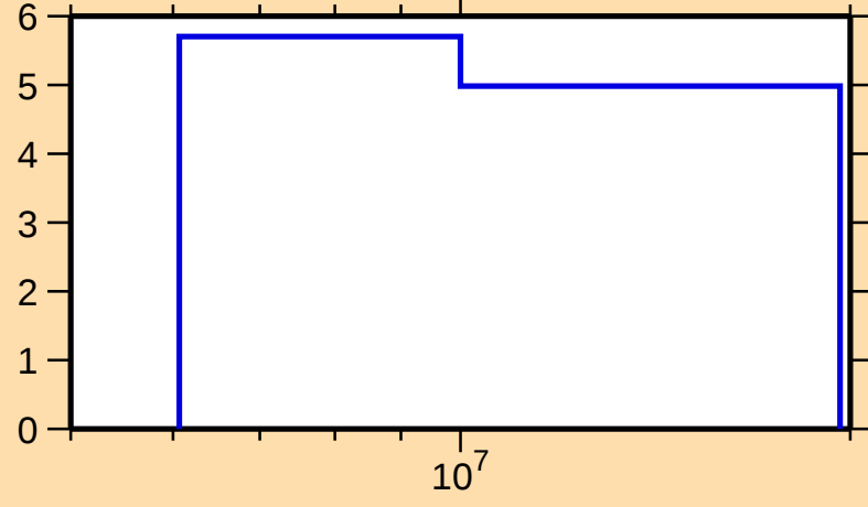
\Delta\sigma/\sigma vs. E for ^{164}\text{Yb}(n,\text{nonel.})
