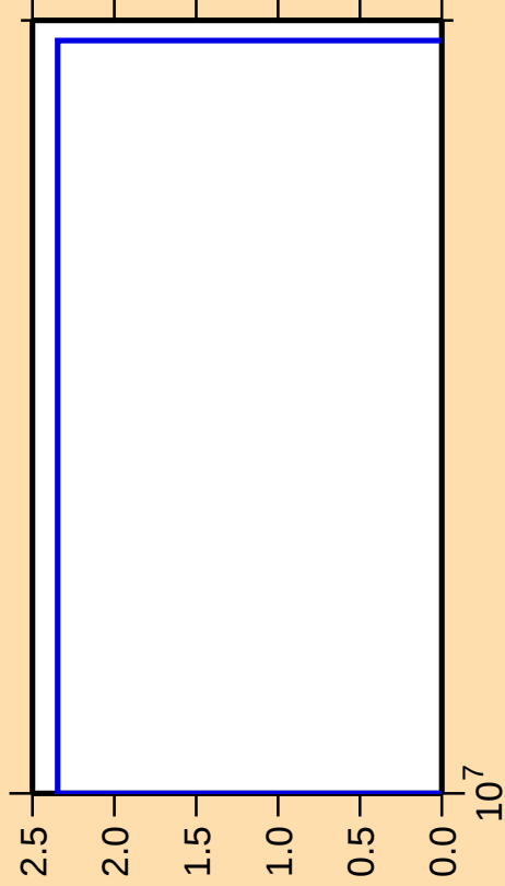
\Delta\sigma/\sigma vs. E for ^{164}\text{Yb}(\text{mt117})
