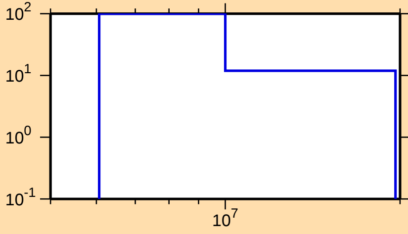
\Delta\sigma/\sigma vs. E for ^{164}\text{Yb}(n,2n)
