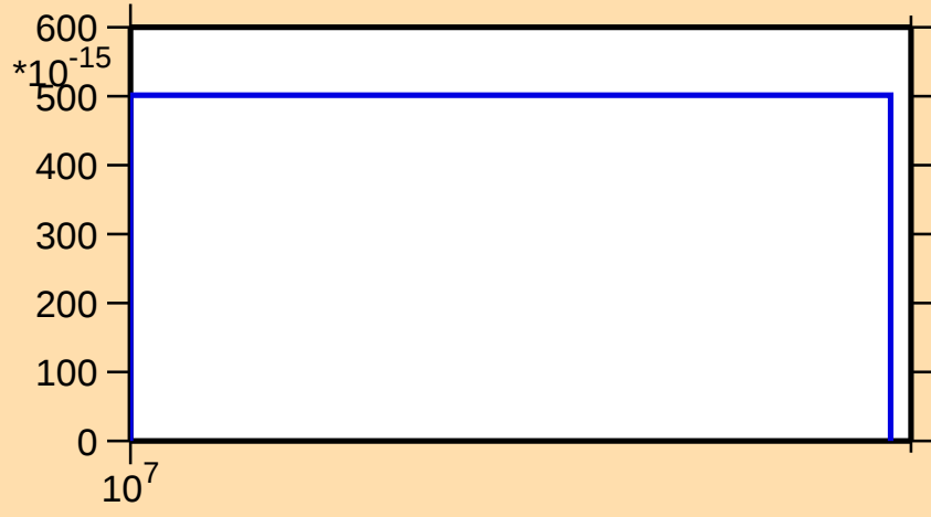
\sigma vs. E for ^{164}\text{Yb}(\text{mt117})
