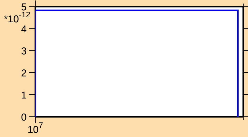
\sigma vs. E for ^{164}\text{Yb} (mt 45)
