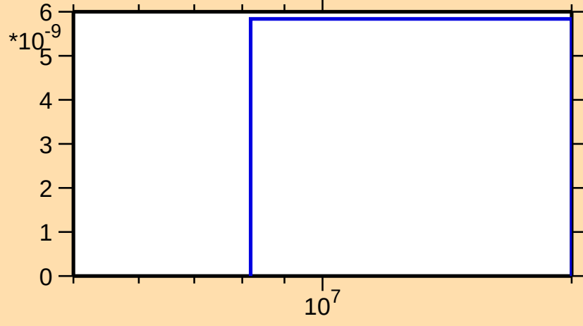
\sigma vs. E for ^{164}\text{Yb}(n,\text{He}3)
