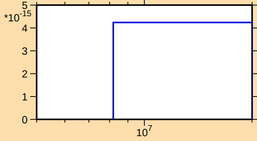
\sigma vs. E for ^{164}\text{Yb}(n,\text{pt})
