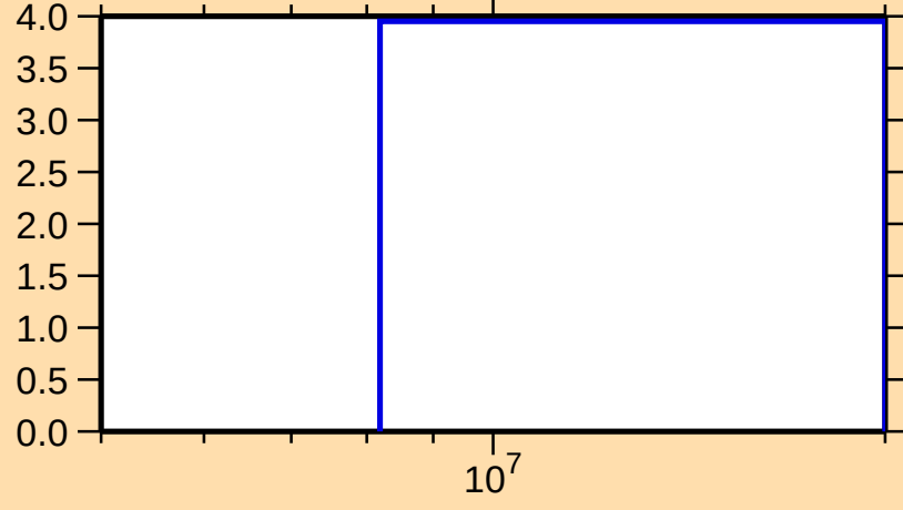
\Delta\sigma/\sigma vs. E for ^{164}\text{Yb}(n,\text{el.})
