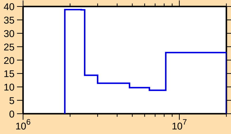
\Delta\sigma/\sigma vs. E for ^{164}\text{Yb}(n,n\text{cont.})
