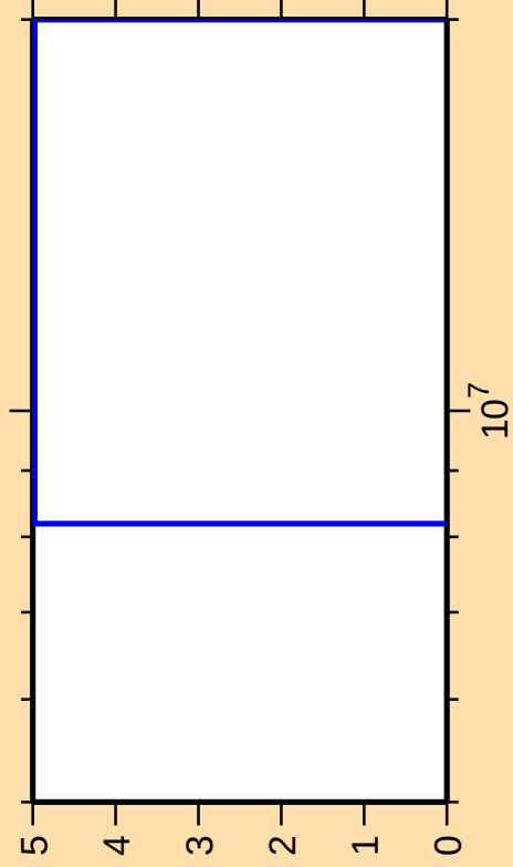
\Delta\sigma/\sigma vs. E for ^{164}\text{Yb}(n,nt)
