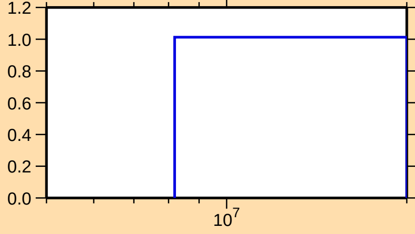
\sigma vs. E for ^{164}\text{Yb}(n,2n)
