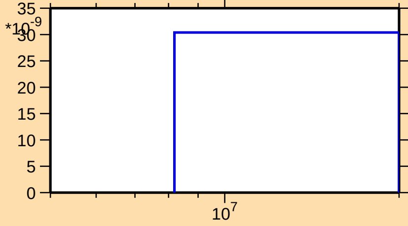
\sigma vs. E for ^{164}\text{Yb}(n,2n\alpha)
