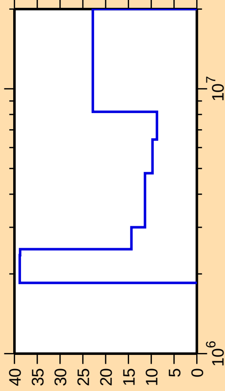
\Delta\sigma/\sigma vs. E for ^{164}\text{Yb}(n,\text{ncont.})
