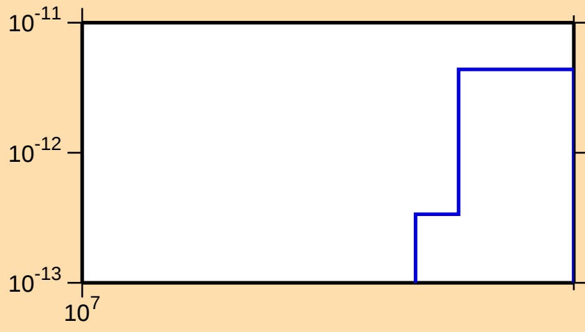
\sigma vs. E for ^{165}\text{Yb}(\text{mt117})
