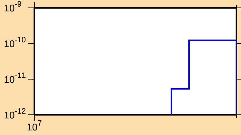
\sigma vs. E for ^{165}\text{Yb}(n,\text{pd})
