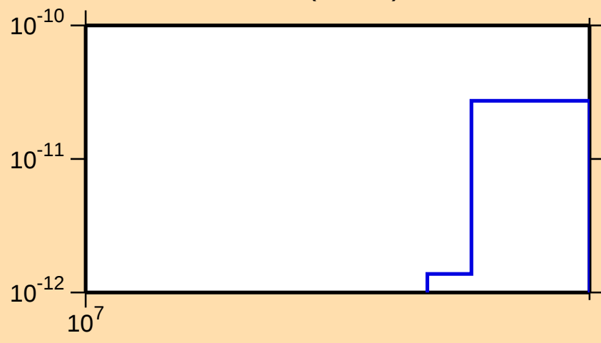
\sigma vs. E for ^{165}\text{Yb} (mt 45)
