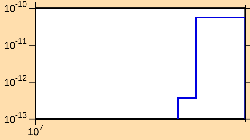
\sigma vs. E for ^{165}\text{Yb}(n,\text{pt})
