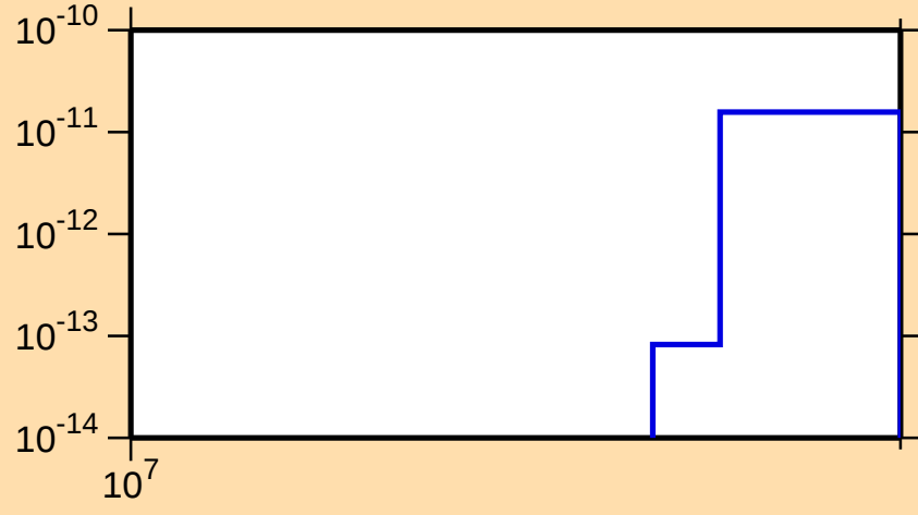
\sigma vs. E for ^{165}\text{Yb} (mt 34)
