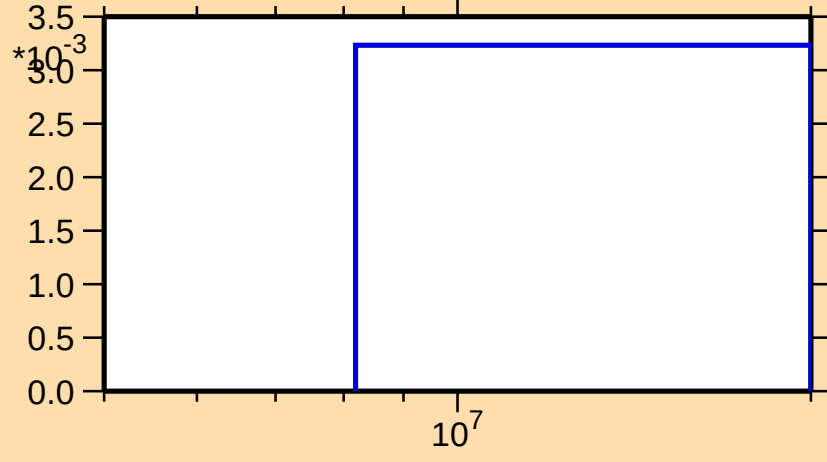
\sigma vs. E for ^{169}\text{Yb}(n,3n)
