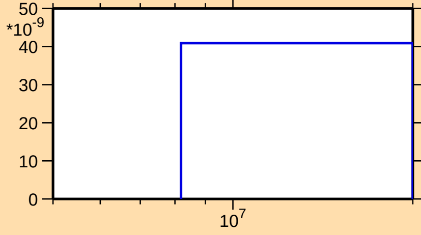
\sigma vs. E for ^{169}\text{Yb}(n,\text{nd})
