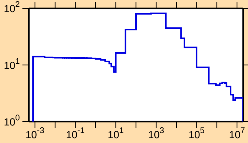
\sigma vs. E for ^{169}\text{Yb}(n,\text{el.})
