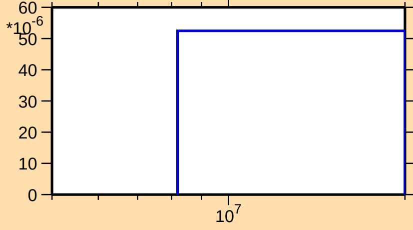
\sigma vs. E for ^{169}\text{Yb}(n,t)
