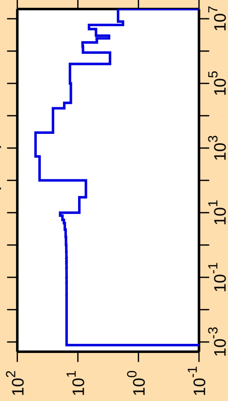
\Delta\sigma/\sigma vs. E for ^{169}\text{Yb}(n,\text{el.})
