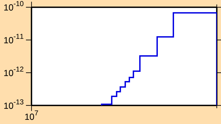
\sigma vs. E for ^{170}\text{Yb}(n,p\alpha)
