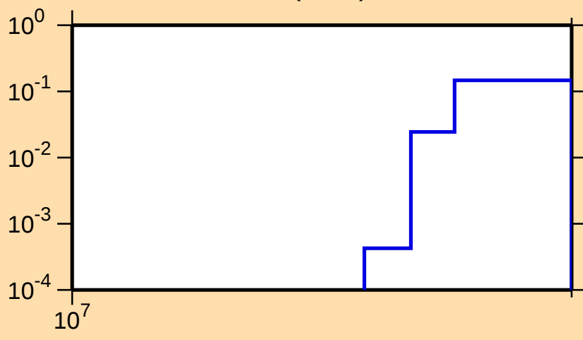
\sigma vs. E for ^{170}\text{Yb}(n,3n)
