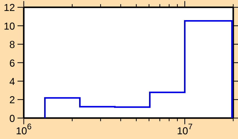
\Delta\sigma/\sigma vs. E for ^{170}\text{Yb}(n,\text{inel.})
