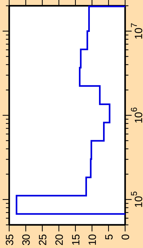
\Delta\sigma/\sigma vs. E for ^{170}\text{Yb}(n,n_1)
