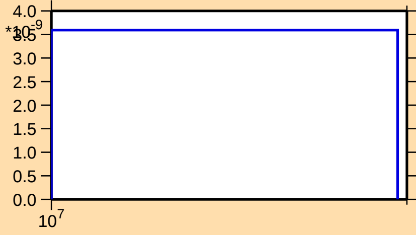
\sigma vs. E for ^{170}\text{Yb}(n,2n\alpha)
