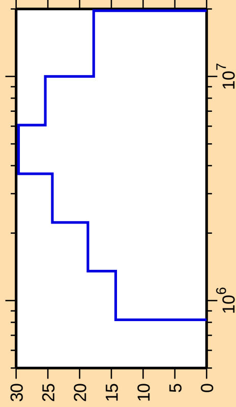
\Delta\sigma/\sigma vs. E for ^{170}\text{Yb}(n,n_4)
