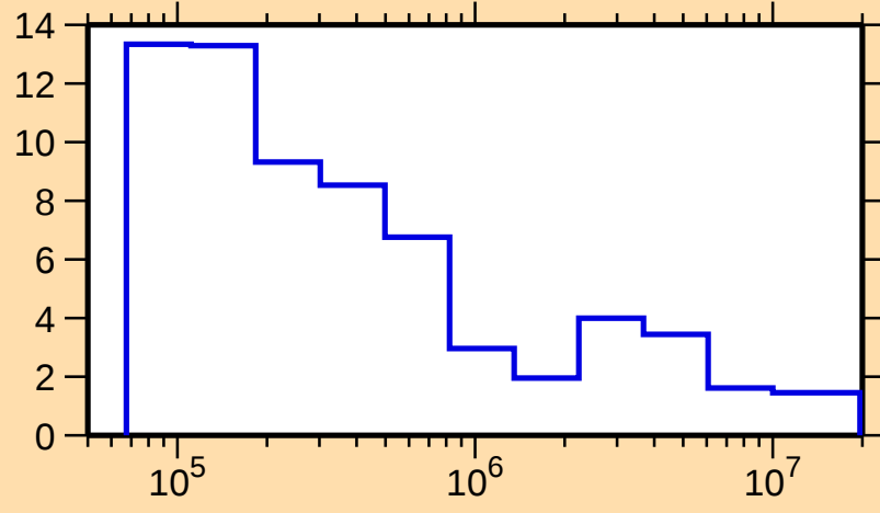
\Delta\sigma/\sigma vs. E for ^{170}\text{Yb}(n,\text{el.})
