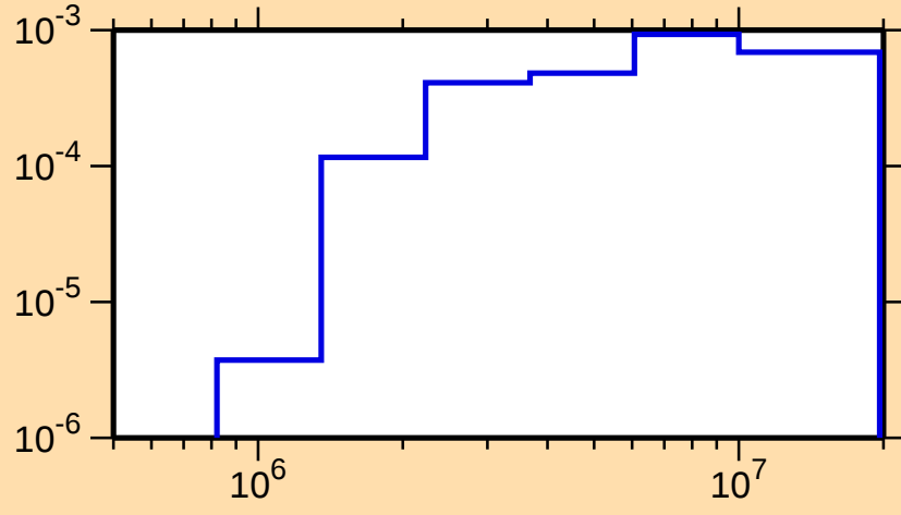
\sigma vs. E for ^{170}\text{Yb}(n,n_4)
