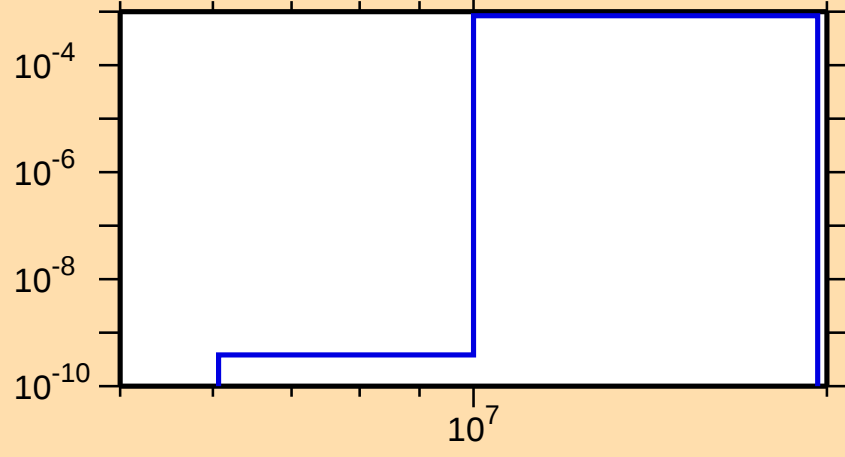
\sigma vs. E for ^{170}\text{Yb}(n,np)
