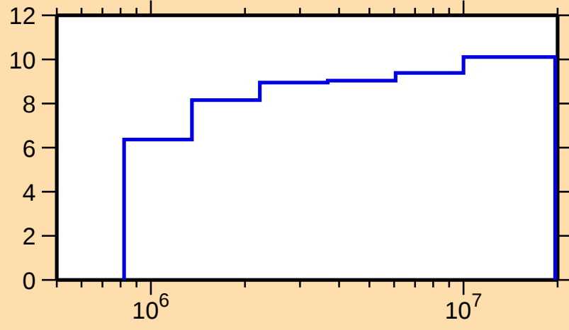
\Delta\sigma/\sigma vs. E for ^{173}\text{Yb}(n, n_1)
