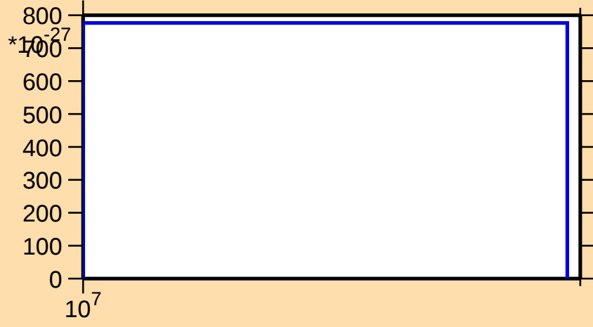
\sigma vs. E for ^{173}\text{Yb}(\text{mt } 11)
