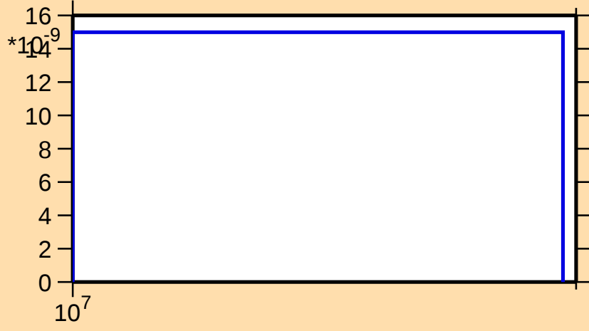
\sigma vs. E for ^{173}\text{Yb}(n,\text{nd})
