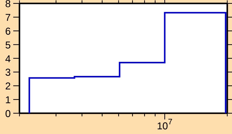
\Delta\sigma/\sigma vs. E for ^{173}\text{Yb}(n,n\text{cont.})
