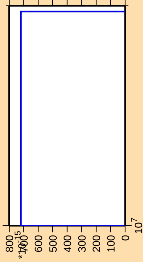
\Delta\sigma/\sigma vs. E for ^{173}\text{Yb}(\text{mt } 11)
