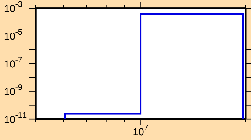
\sigma vs. E for ^{173}\text{Yb}(n,d)
