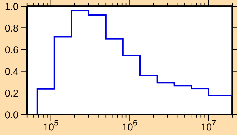
\sigma vs. E for ^{173}\text{Yb}(n,n_1)
