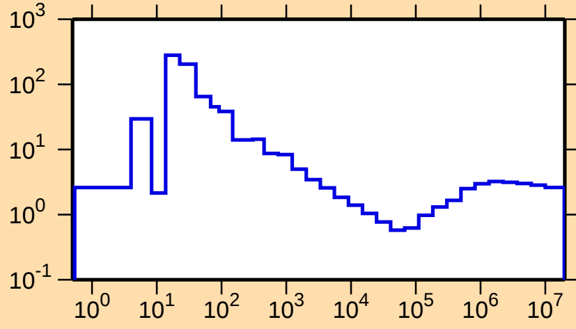
\sigma vs. E for ^{173}\text{Yb}(n,\text{nonel.})
