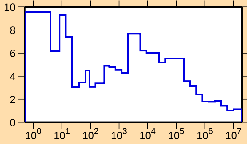
\Delta\sigma/\sigma vs. E for ^{173}\text{Yb}(n,\text{tot.})
