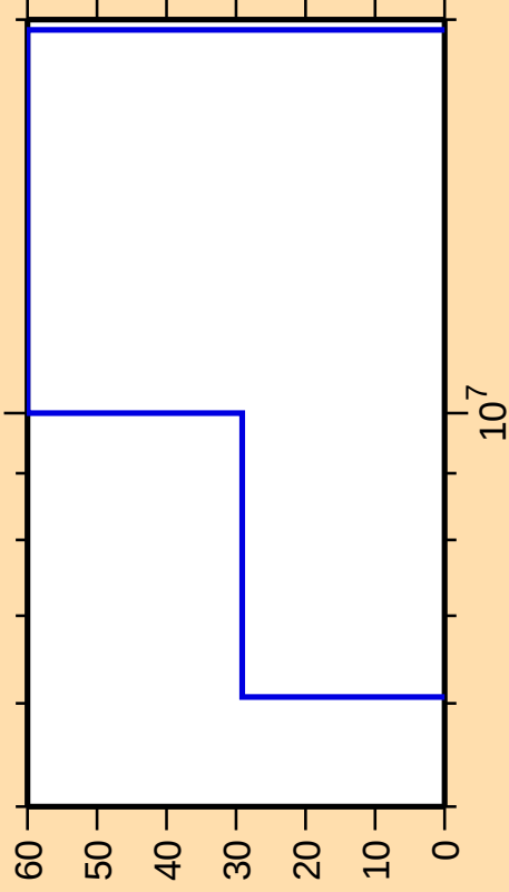
\Delta\sigma/\sigma vs. E for ^{173}\text{Yb}(n,d)
