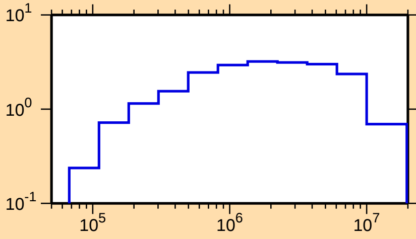
\sigma vs. E for ^{173}\text{Yb}(n,\text{inel.})
