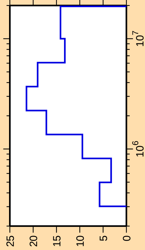
\Delta\sigma/\sigma vs. E for ^{173}\text{Yb}(n,n_4)
