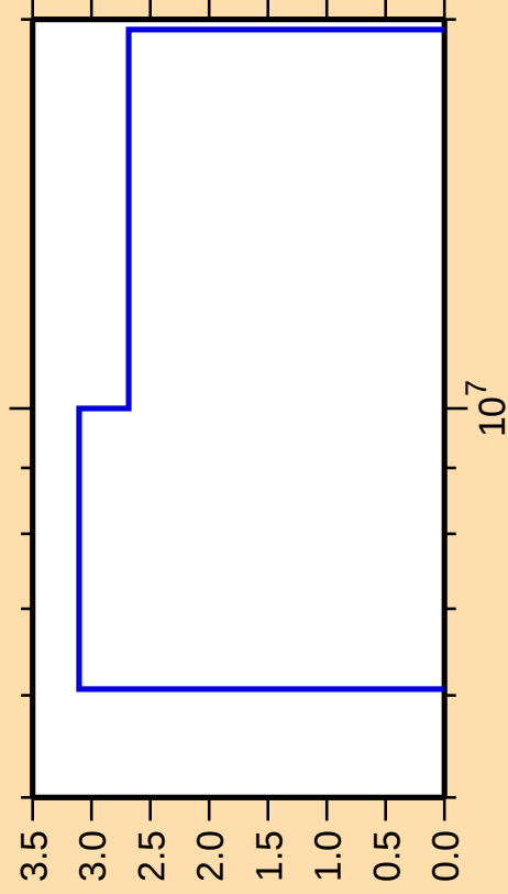
\Delta\sigma/\sigma vs. E for ^{173}\text{Yb}(n,2n)
