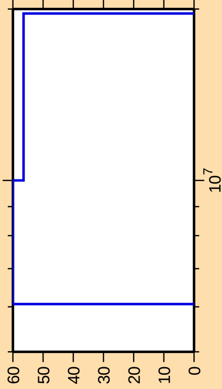
\Delta\sigma/\sigma vs. E for ^{173}\text{Yb}(n,\alpha)
