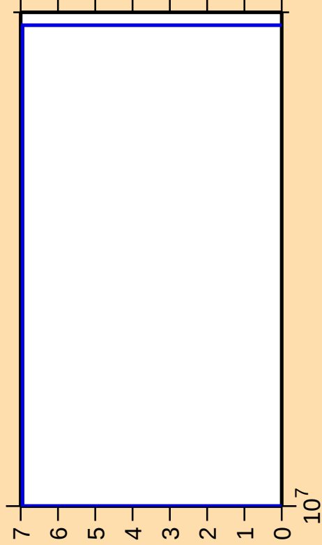
\Delta\sigma/\sigma vs. E for ^{173}\text{Yb}(n,3n)
