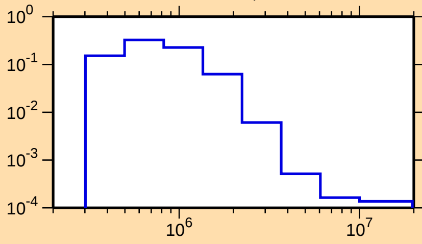
\sigma vs. E for ^{173}\text{Yb}(n,n_4)
