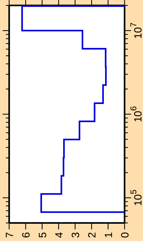
\Delta\sigma/\sigma vs. E for ^{173}\text{Yb}(n,\text{inel.})
