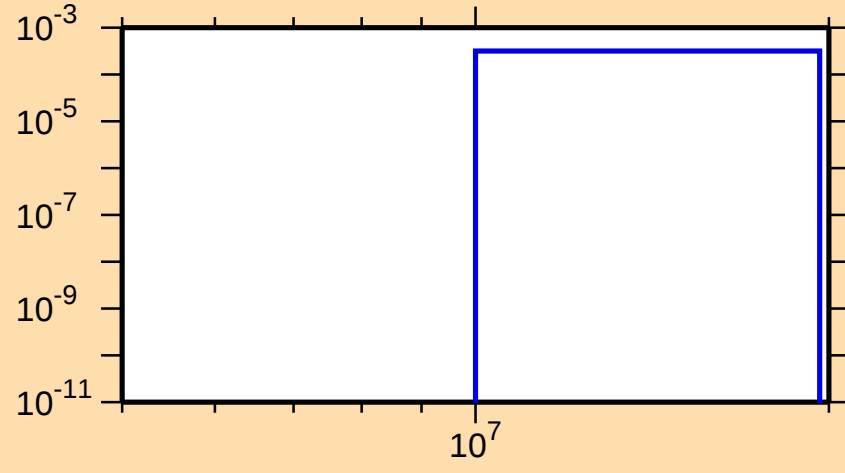
\sigma vs. E for ^{173}\text{Yb}(n,np)
