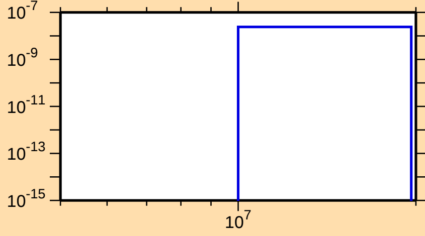
\sigma vs. E for ^{173}\text{Yb}(n,2n\alpha)
