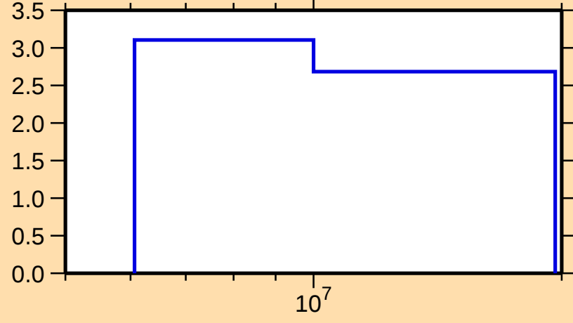
\Delta\sigma/\sigma vs. E for ^{173}\text{Yb}(n,2n)
