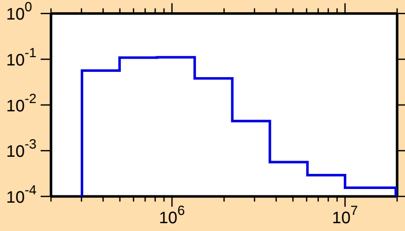
\sigma vs. E for ^{173}\text{Yb}(n,n_3)
