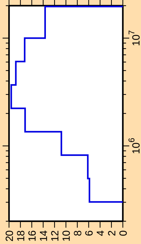
\Delta\sigma/\sigma vs. E for ^{173}\text{Yb}(n,n_3)
