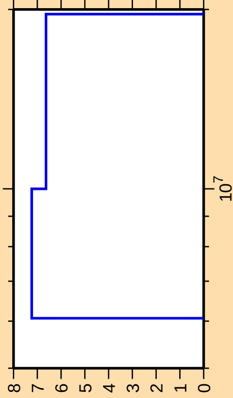
\Delta\sigma/\sigma vs. E for ^{176}\text{Yb}(n,n_1)
