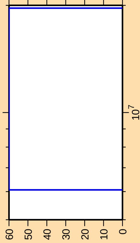
\Delta\sigma/\sigma vs. E for ^{176}\text{Yb}(n,n\alpha)
