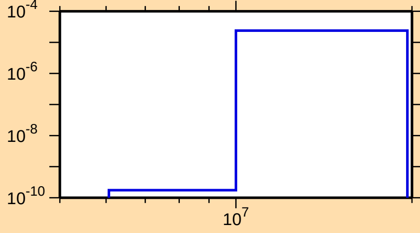
\sigma vs. E for ^{176}\text{Yb}(n,n\alpha)
