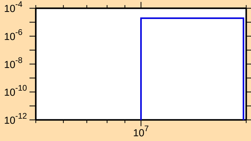
\sigma vs. E for ^{176}\text{Yb}(n,t)
