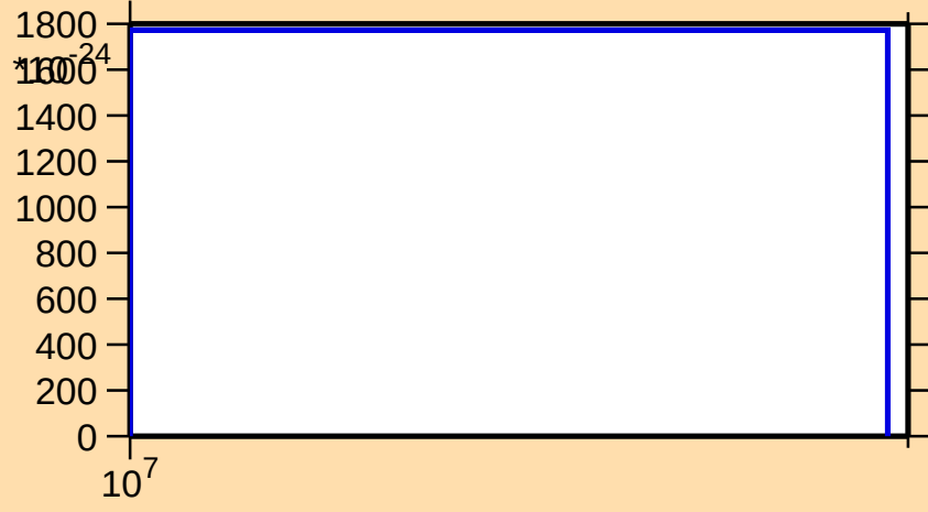
\sigma vs. E for ^{176}\text{Yb} (mt 11)
