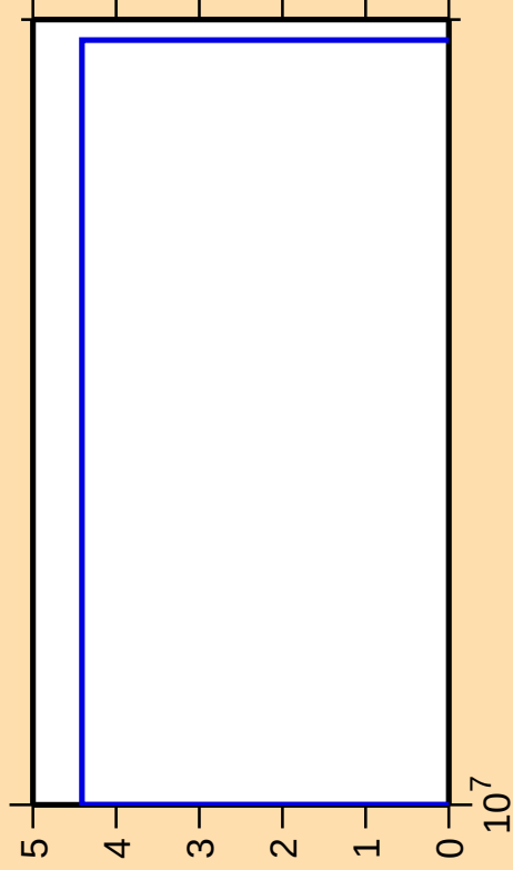
\Delta\sigma/\sigma vs. E for ^{176}\text{Yb}(n,2np)
