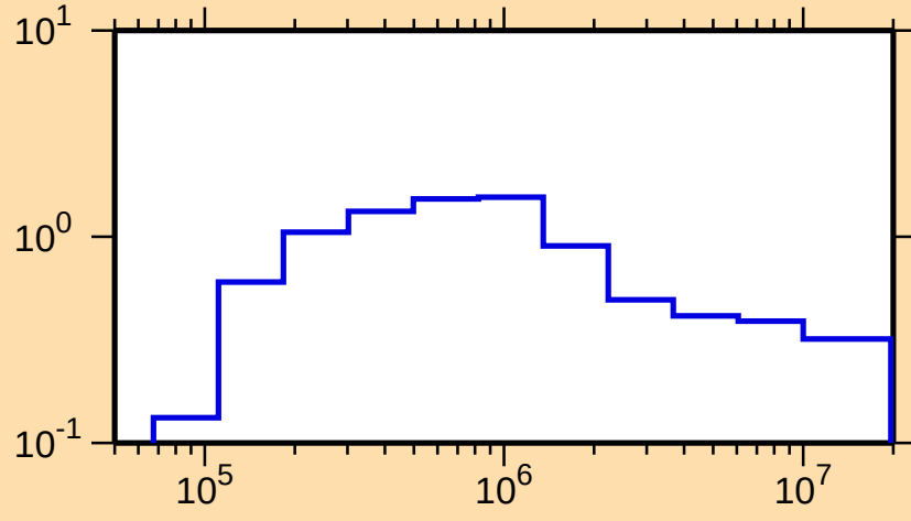
\sigma vs. E for ^{176}\text{Yb}(n,n_1)
