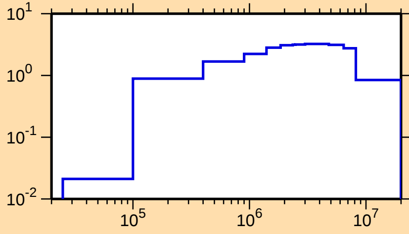
\sigma vs. E for ^{176}\text{Yb}(n,\text{inel.})
