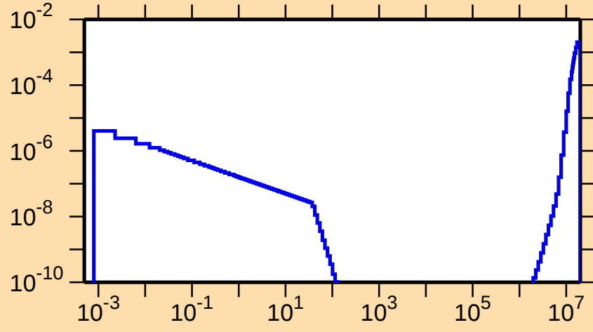
\sigma vs. E for ^{176}\text{Yb}(n,\alpha)
