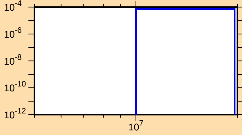
\sigma vs. E for ^{176}\text{Yb}(n,t)
