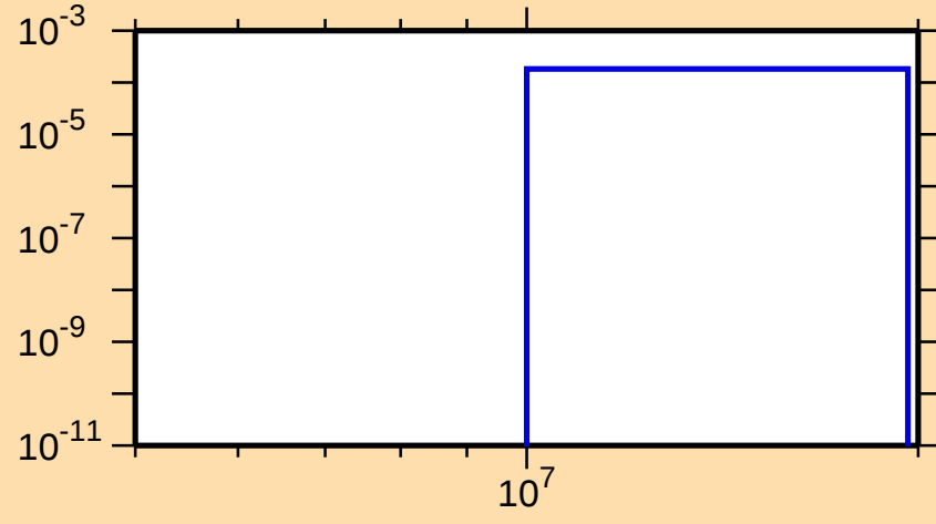
\sigma vs. E for ^{176}\text{Yb}(n,d)
