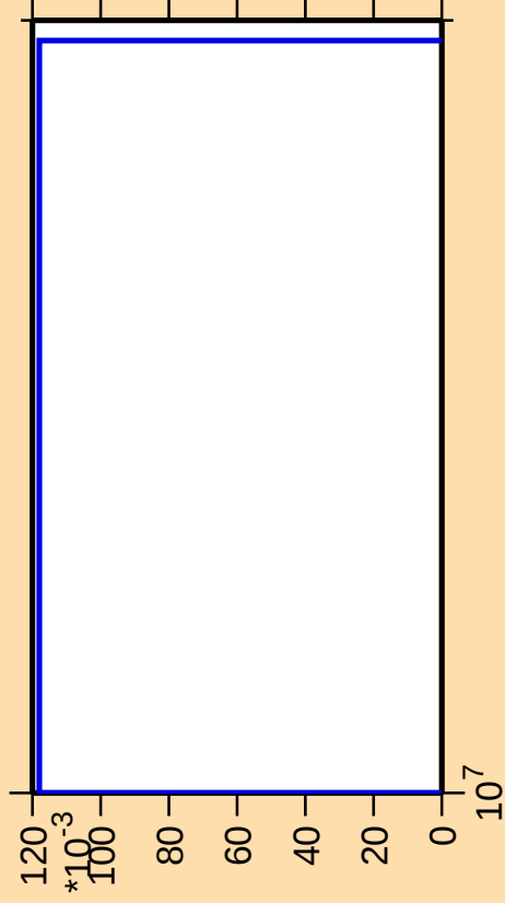
\Delta\sigma/\sigma vs. E for ^{176}\text{Yb}(n,\text{He3})
