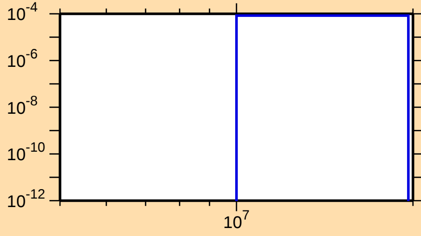
\sigma vs. E for ^{176}\text{Yb}(n,np)
