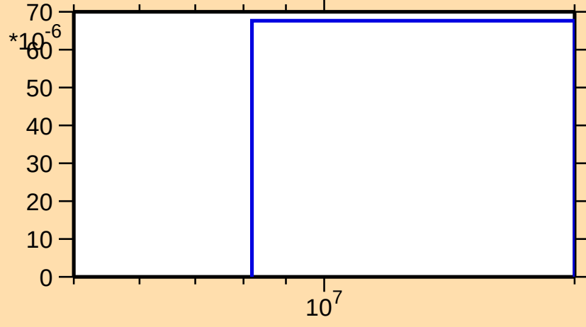
\sigma vs. E for ^{176}\text{Yb}(n,np)
