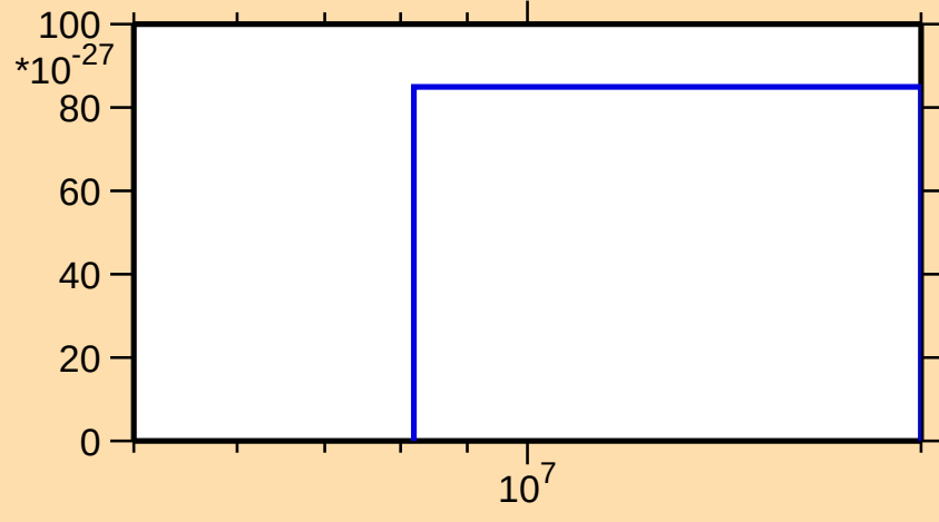
\sigma vs. E for ^{176}\text{Yb} (mt 42)
