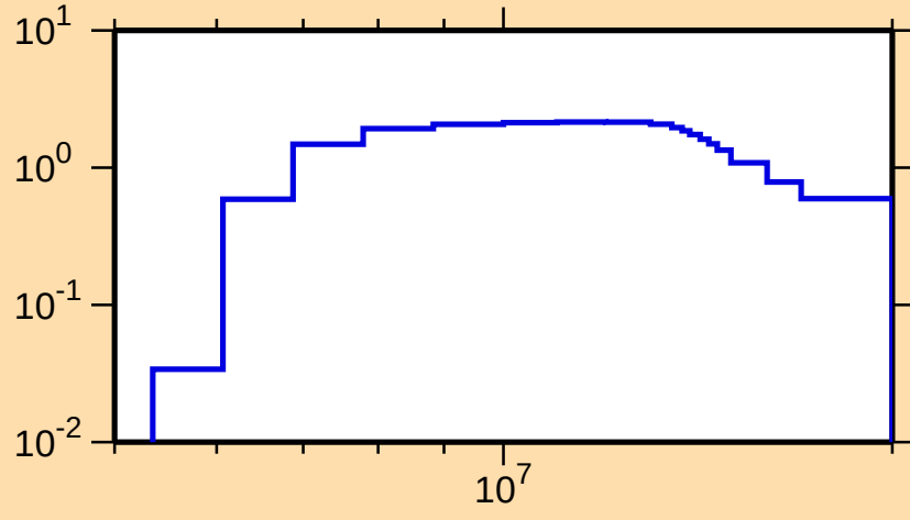
\sigma vs. E for ^{177}\text{Yb}(n,2n)
