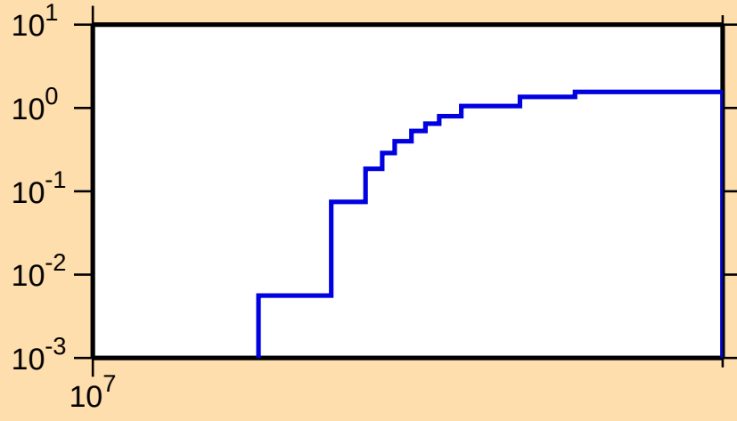
\sigma vs. E for ^{177}\text{Yb}(n,3n)
