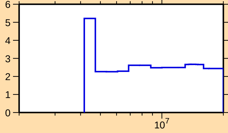
\Delta\sigma/\sigma vs. E for ^{177}\text{Yb}(n,\text{nonel.})
