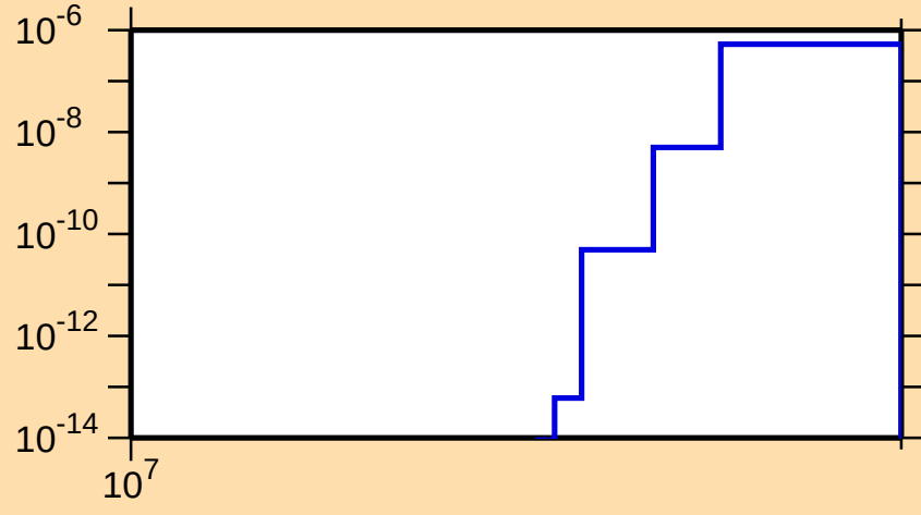
\sigma vs. E for ^{177}\text{Yb}(n,\text{nd})
