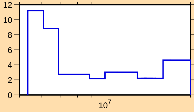
\Delta\sigma/\sigma vs. E for ^{177}\text{Yb}(n,\text{el.})
