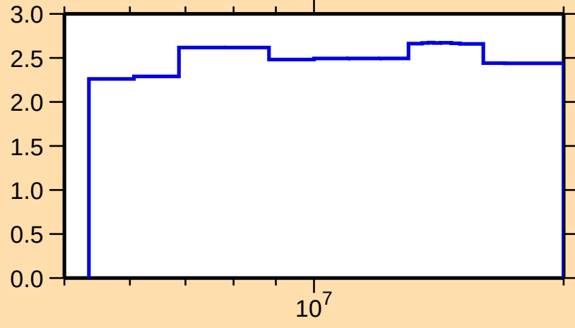
\Delta\sigma/\sigma vs. E for ^{177}\text{Yb}(n,\text{nonel.})
