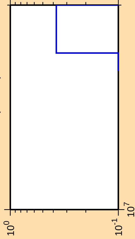
\Delta\sigma/\sigma vs. E for ^{177}\text{Yb}(n,\text{He3})
