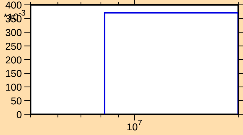
\sigma vs. E for ^{177}\text{Yb}(n,3n)
