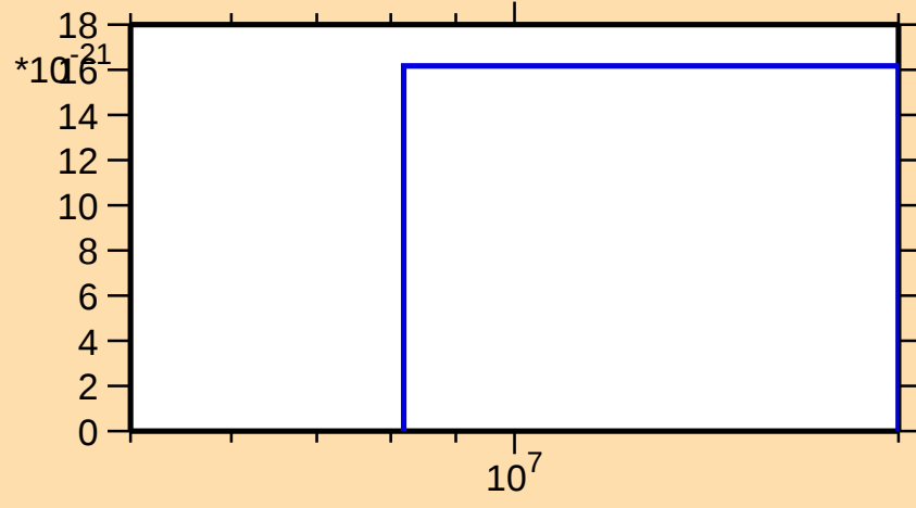
\sigma vs. E for ^{177}\text{Yb} (mt 11)
