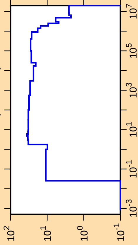
\Delta\sigma/\sigma vs. E for ^{177}\text{Yb}(n,\text{nonel.})
