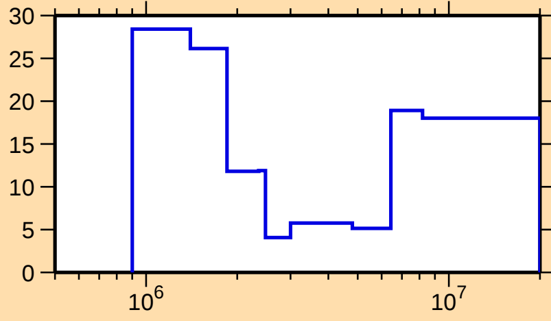
\Delta\sigma/\sigma vs. E for ^{177}\text{Yb}(n,n\text{cont.})
