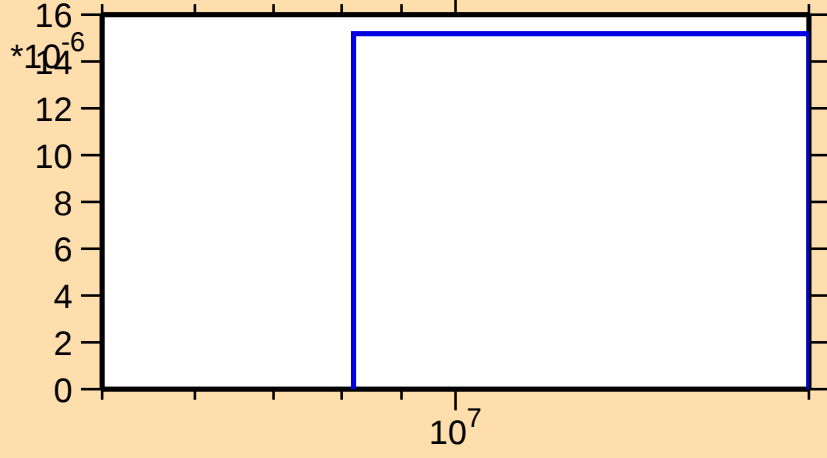
\sigma vs. E for ^{177}\text{Yb}(n,t)
