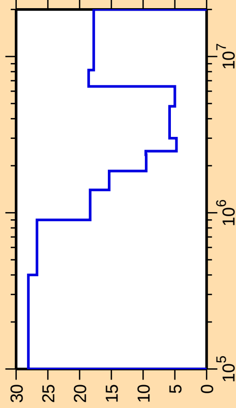
\Delta\sigma/\sigma vs. E for ^{177}\text{Yb}(n,\text{inel.})
