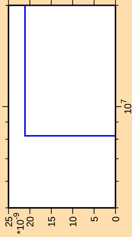
\Delta\sigma/\sigma vs. E for ^{177}\text{Yb} (mt 11)
