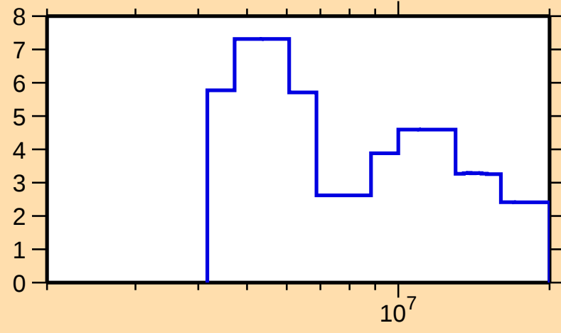
\Delta\sigma/\sigma vs. E for ^{177}\text{Yb}(n,\text{el.})
