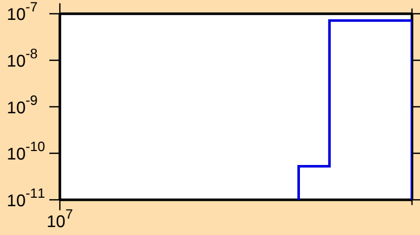
\sigma vs. E for ^{177}\text{Yb}(n,2np)
