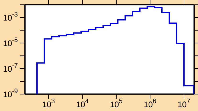
\sigma vs. E for ^{177}\text{Yb}(n,n_3)
