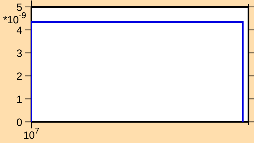
\sigma vs. E for ^{177}\text{Yb}(n,nt)
