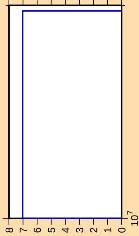
\Delta\sigma/\sigma vs. E for ^{177}\text{Yb}(n,3n)
