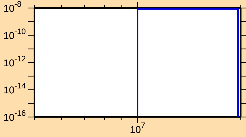
\sigma vs. E for ^{177}\text{Yb}(n,2n\alpha)
