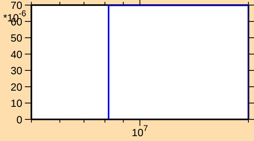
\sigma vs. E for ^{177}\text{Yb}(n,d)
