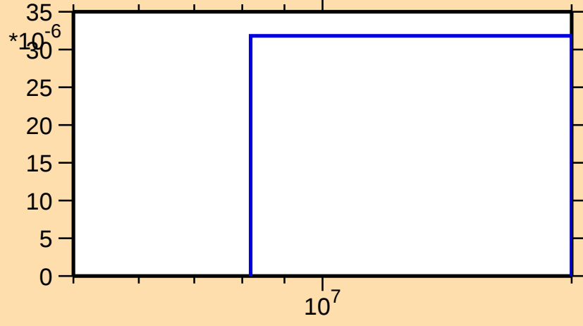
\sigma vs. E for ^{177}\text{Yb}(n,np)
