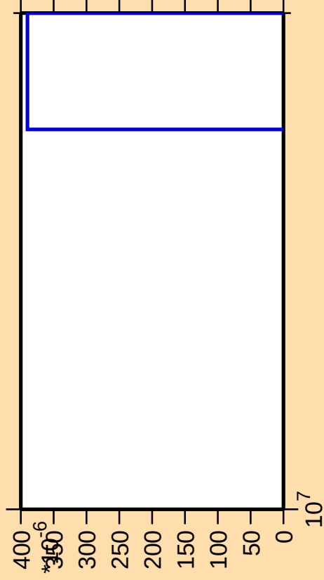
\Delta\sigma/\sigma vs. E for ^{181}\text{Yb}(\text{mt } 11)
