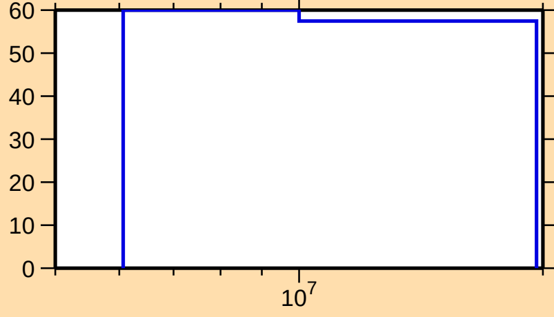
\Delta\sigma/\sigma vs. E for ^{181}\text{Yb}(n,n\text{cont.})
