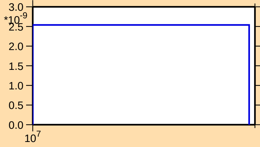
\sigma vs. E for ^{181}\text{Yb}(n,\text{nd})
