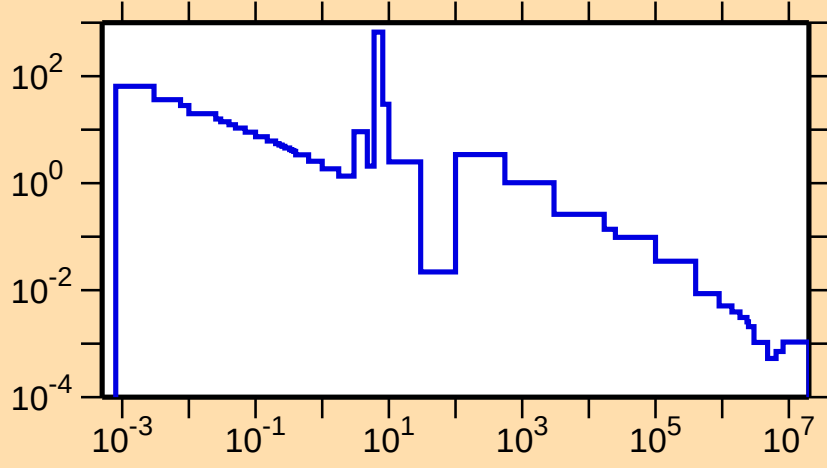
\sigma vs. E for ^{181}\text{Yb}(n,\gamma)
