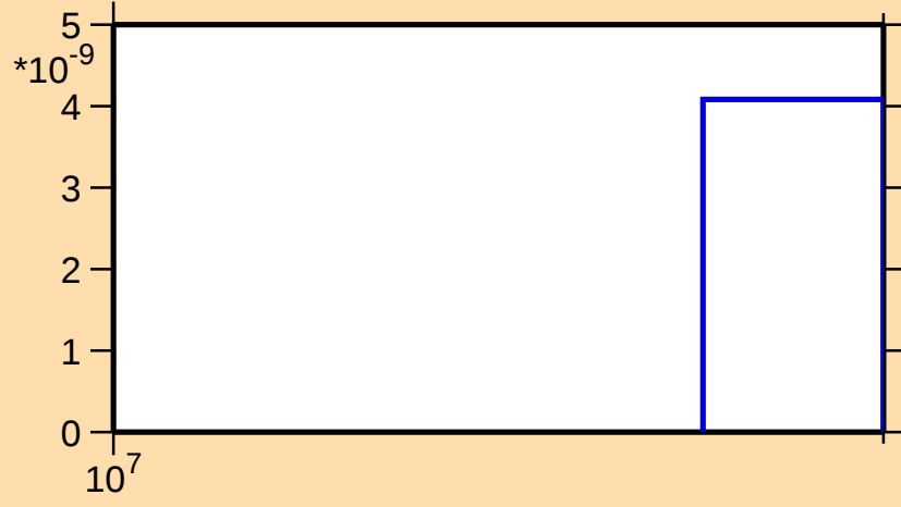
\sigma vs. E for ^{62}\text{Zn}(n,2np)
