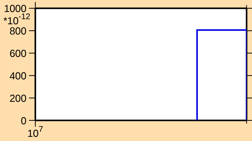
\sigma vs. E for ^{69}\text{Zn}(n,\text{nt})
