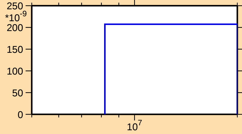
\sigma vs. E for ^{69}\text{Zn}(n,2n\alpha)
