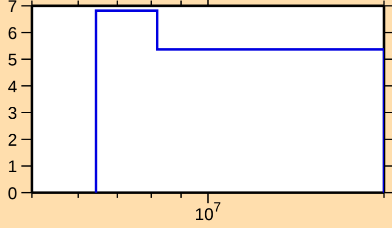
\Delta\sigma/\sigma vs. E for ^{69}\text{Zn}(n,2n)
