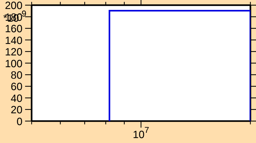
\sigma vs. E for ^{69}\text{Zn}(n,\text{nd})
