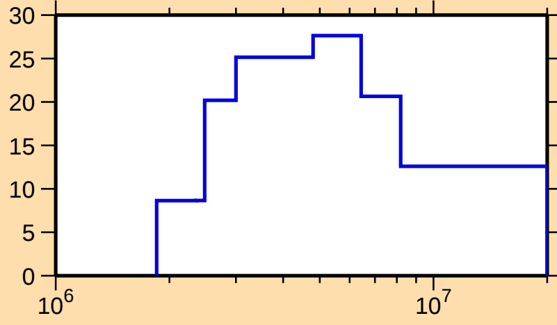
\Delta\sigma/\sigma vs. E for ^{69}\text{Zn}(n,n_1)
