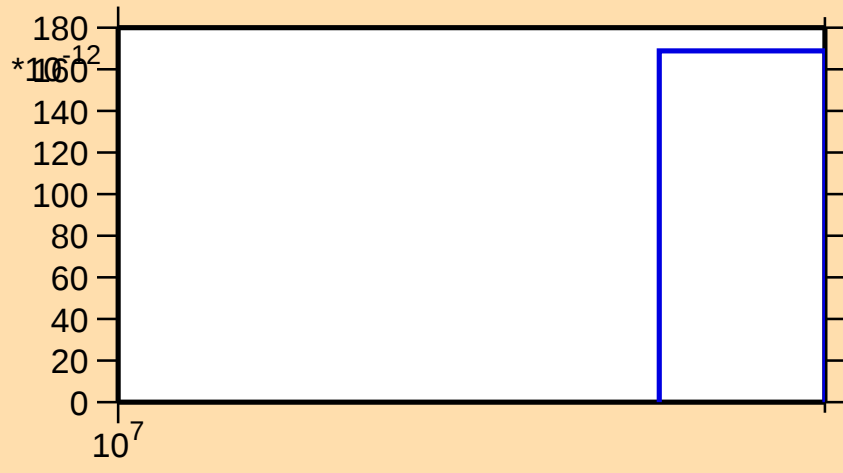
\sigma vs. E for ^{72}\text{Zn}(n,nt)
