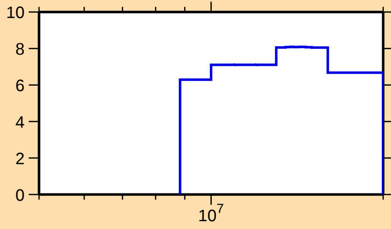
\Delta\sigma/\sigma vs. E for ^{72}\text{Zn}(n,\text{el.})
