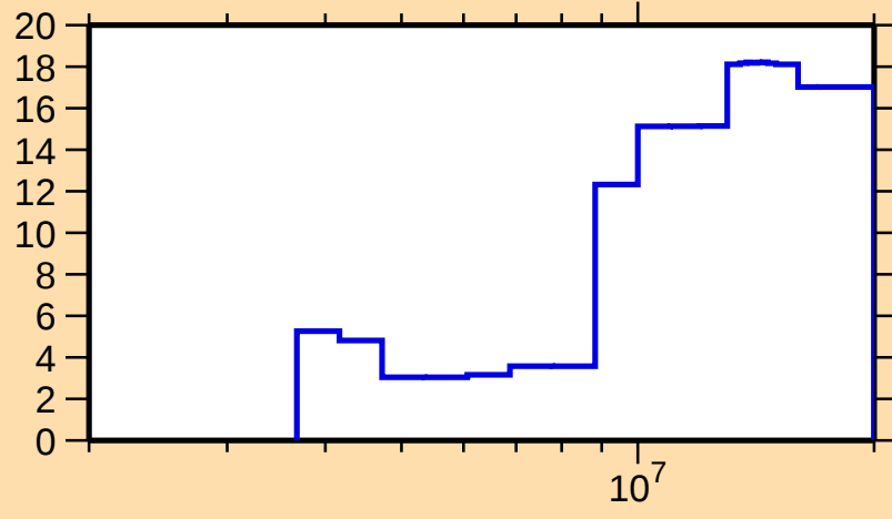
\Delta\sigma/\sigma vs. E for ^{72}\text{Zn}(n,\text{inel.})
