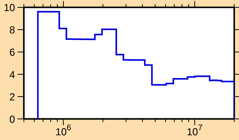
\Delta\sigma/\sigma vs. E for ^{72}\text{Zn}(n,\text{nonel.})
