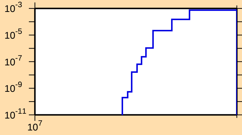
\sigma vs. E for ^{72}\text{Zn}(n,np)
