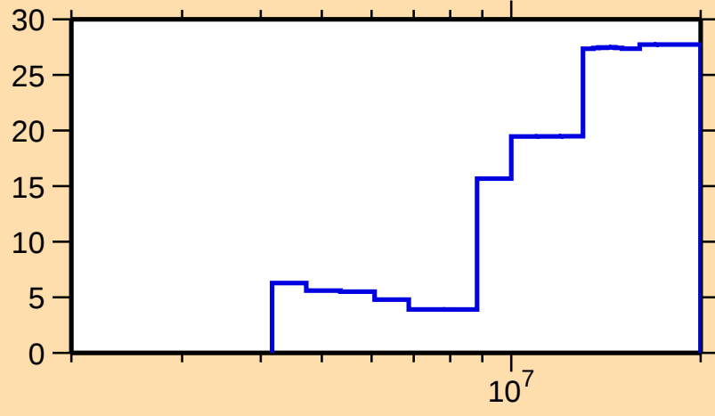
\Delta\sigma/\sigma vs. E for ^{72}\text{Zn}(n,n\text{cont.})
