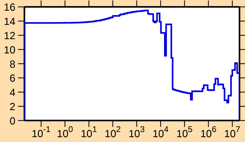
\Delta\sigma/\sigma vs. E for ^{72}\text{Zn}(n,\text{el.})
