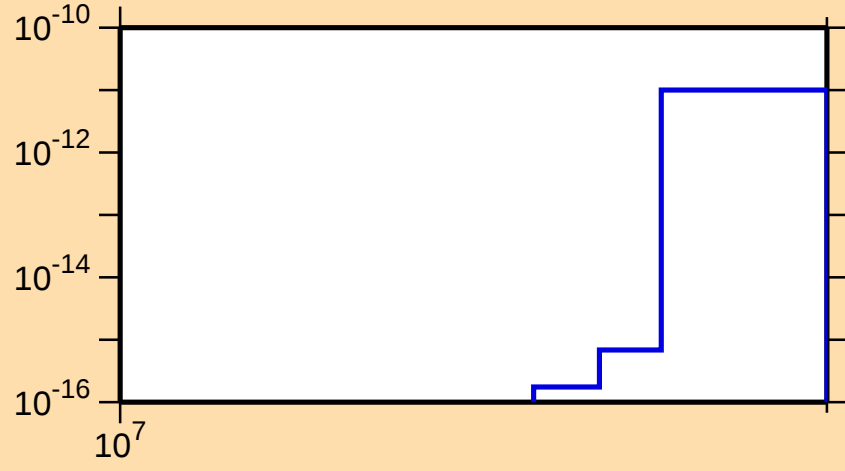
\sigma vs. E for ^{72}\text{Zn}(n,2n\alpha)
