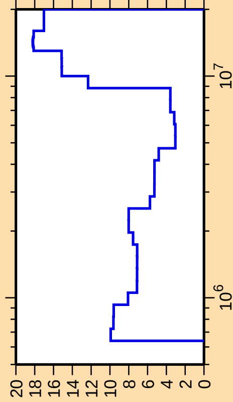
\Delta\sigma/\sigma vs. E for ^{72}\text{Zn}(n,\text{inel.})
