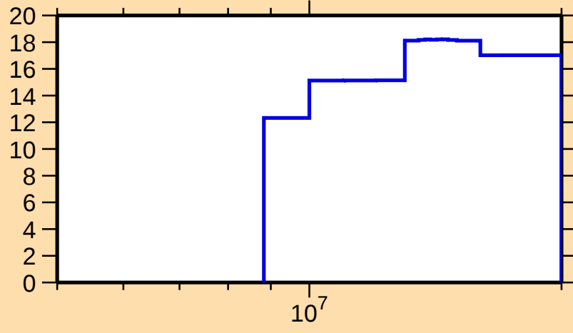
\Delta\sigma/\sigma vs. E for ^{72}\text{Zn}(n,\text{inel.})
