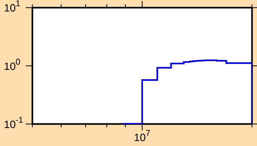
\sigma vs. E for ^{72}\text{Zn}(n,2n)
