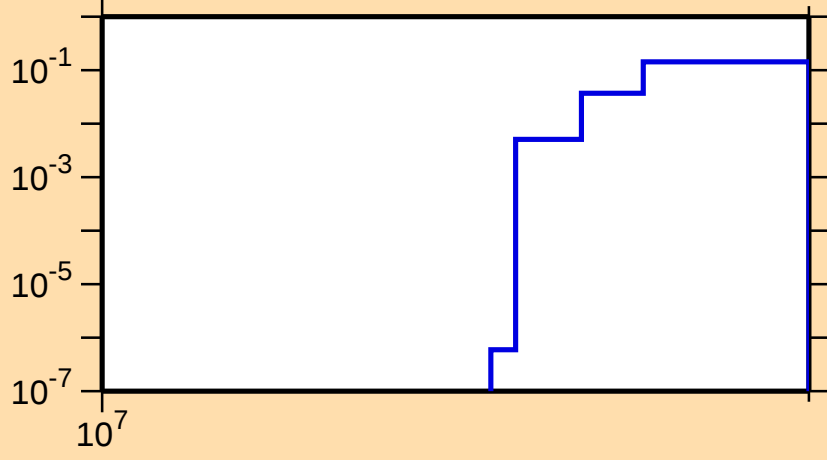
\sigma vs. E for ^{72}\text{Zn}(n,3n)
