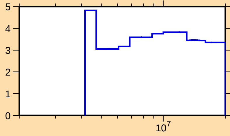
\Delta\sigma/\sigma vs. E for ^{72}\text{Zn}(n,\text{nonel.})
