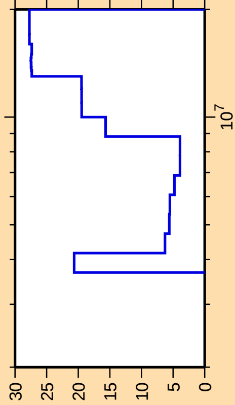
\Delta\sigma/\sigma vs. E for ^{72}\text{Zn}(n,n\text{cont.})
