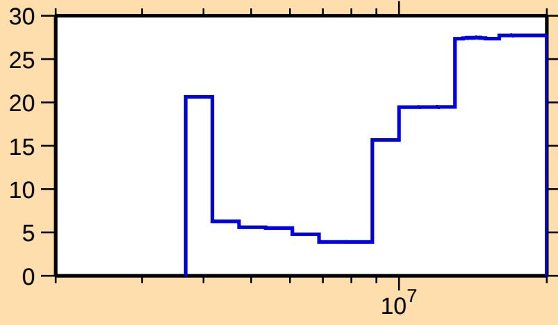
\Delta\sigma/\sigma vs. E for ^{72}\text{Zn}(n,n\text{cont.})
