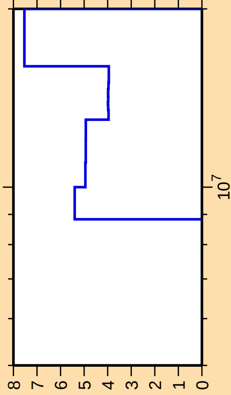
\Delta\sigma/\sigma vs. E for ^{72}\text{Zn}(n,2n)
