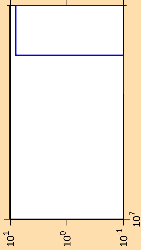
\Delta\sigma/\sigma vs. E for ^{72}\text{Zn}(n,2n\alpha)
