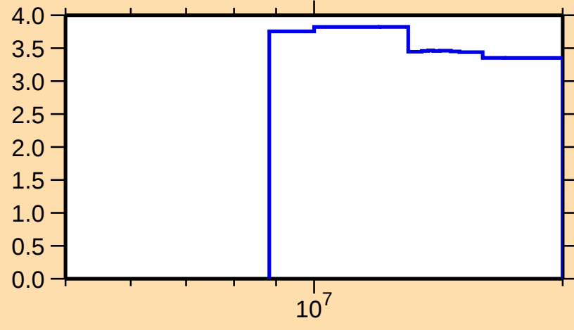
\Delta\sigma/\sigma vs. E for ^{72}\text{Zn}(n,\text{nonel.})
