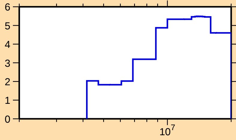
\Delta\sigma/\sigma vs. E for ^{72}\text{Zn}(n,\text{tot.})
