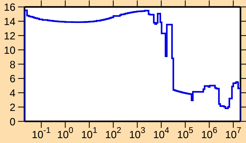
\Delta\sigma/\sigma vs. E for ^{72}\text{Zn}(n,\text{tot.})
