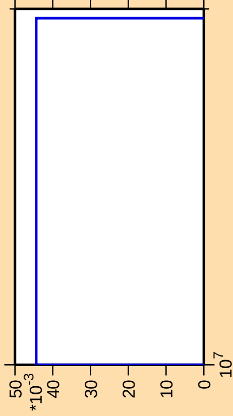
\Delta\sigma/\sigma vs. E for ^{72}\text{Zn}(n,2n\alpha)
