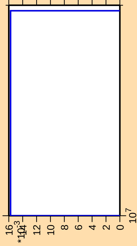
\Delta\sigma/\sigma vs. E for ^{72}\text{Zn}(n,\text{nd})
