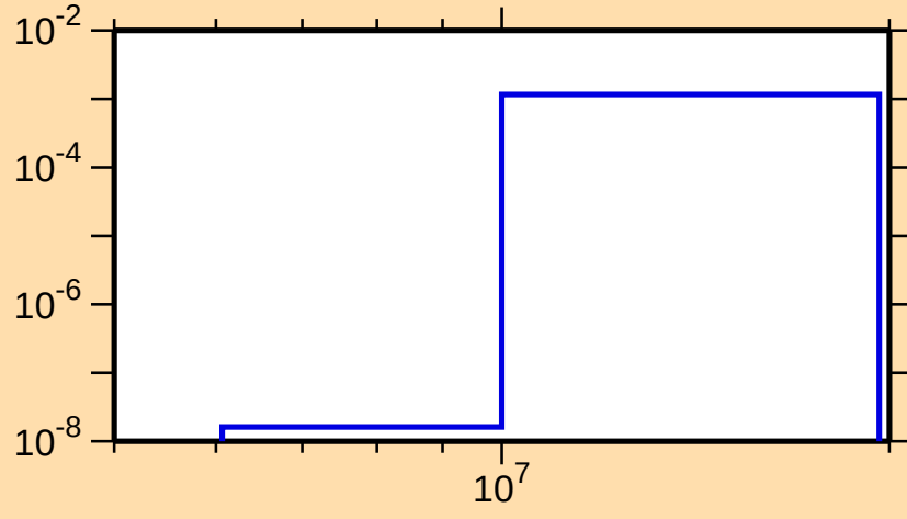
\sigma vs. E for ^{72}\text{Zn}(n,p)
