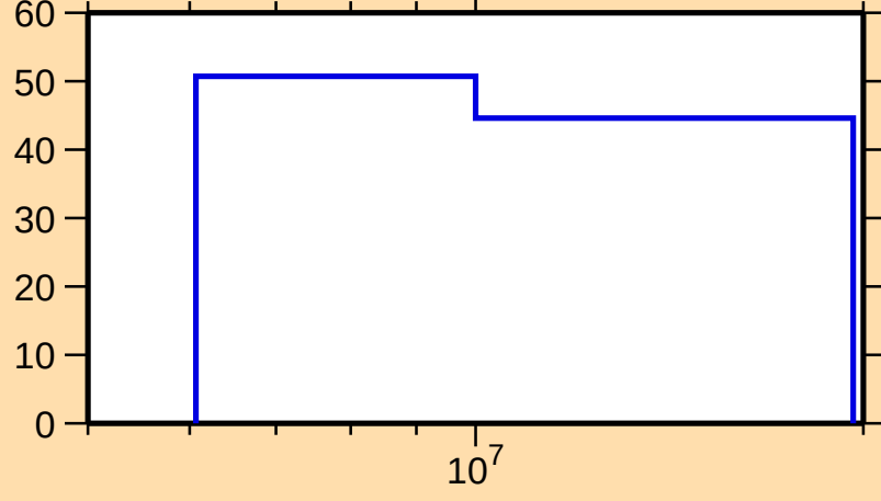
\Delta\sigma/\sigma vs. E for ^{72}\text{Zn}(n,p)
