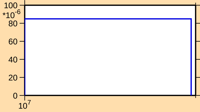
\sigma vs. E for ^{72}\text{Zn}(n,d)
