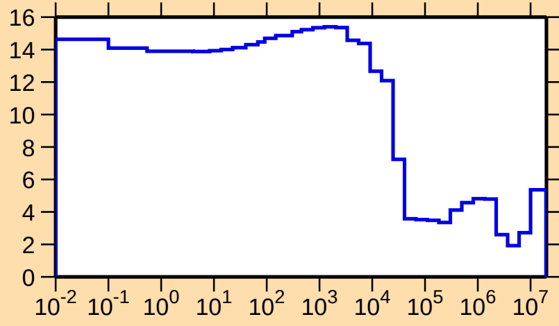
\Delta\sigma/\sigma vs. E for ^{72}\text{Zn}(n,\text{tot.})
