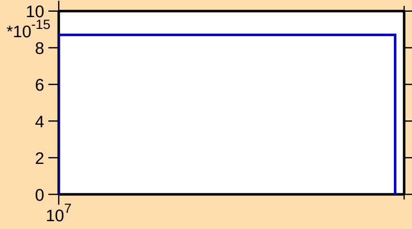
\sigma vs. E for ^{72}\text{Zn}(n,\text{nd})
