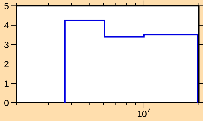
\Delta\sigma/\sigma vs. E for ^{72}\text{Zn}(n,n\text{oncl.})
