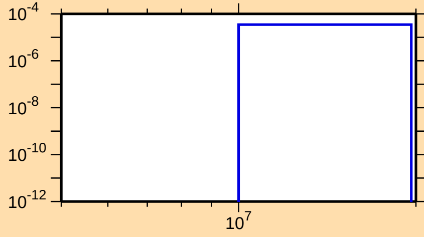
\sigma vs. E for ^{72}\text{Zn}(n,n\alpha)
