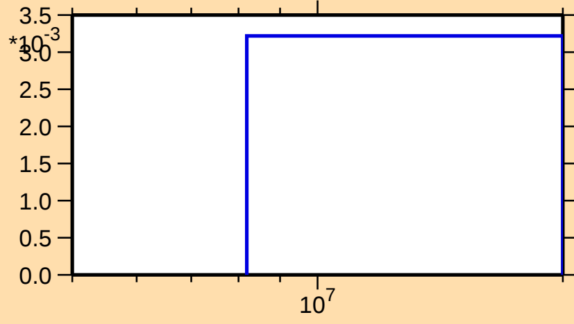
\sigma vs. E for ^{72}\text{Zn}(n,3n)
