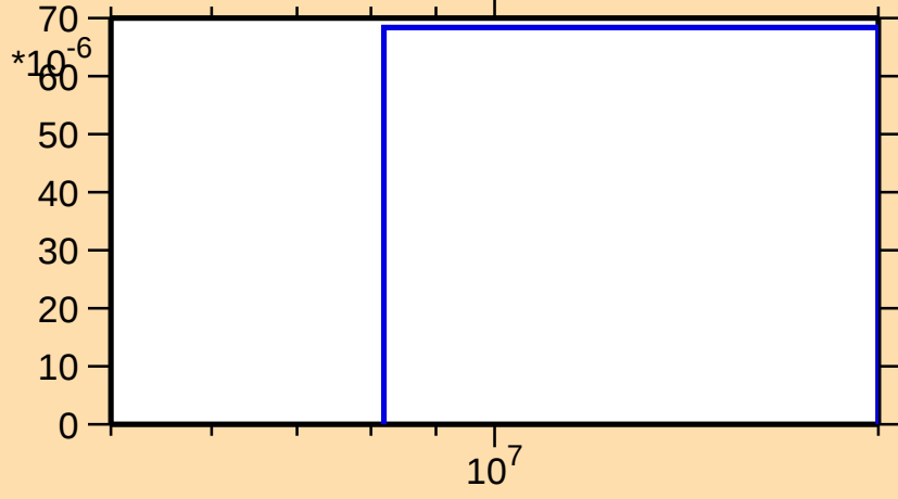
\sigma vs. E for ^{72}\text{Zn}(n,d)
