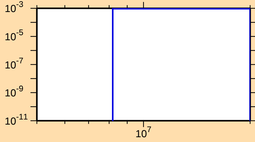
\sigma vs. E for ^{72}\text{Zn}(n,p)
