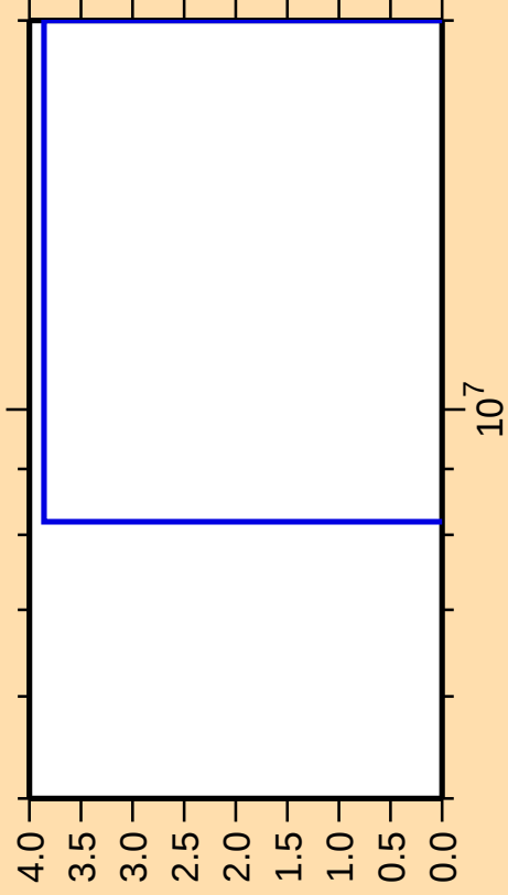
\Delta\sigma/\sigma vs. E for ^{72}\text{Zn}(n,2n)
