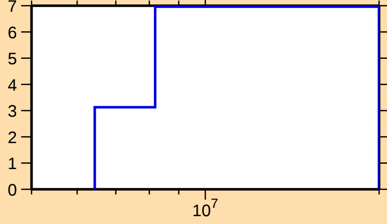
\Delta\sigma/\sigma vs. E for ^{72}\text{Zn}(n,\text{el.})
