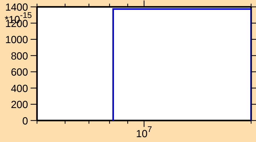
\sigma vs. E for ^{72}\text{Zn}(n,nt)
