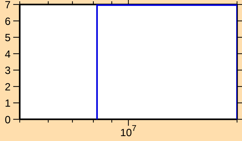
\Delta\sigma/\sigma vs. E for ^{72}\text{Zn}(n,\text{el.})
