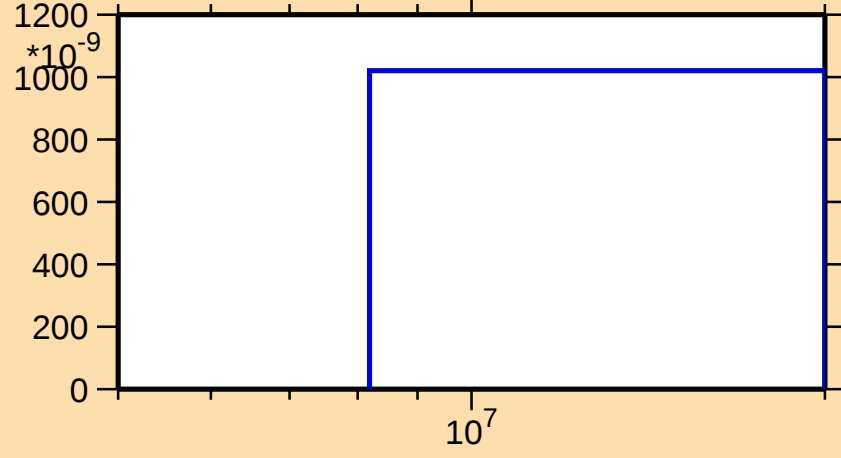
\sigma vs. E for ^{72}\text{Zn}(n,t)
