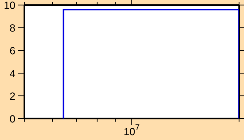
\Delta\sigma/\sigma vs. E for ^{72}\text{Zn}(n,n_1)
