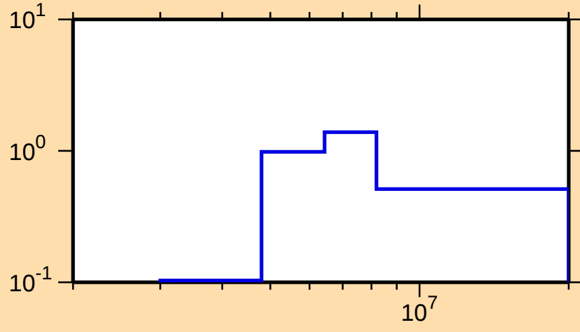
\sigma vs. E for ^{72}\text{Zn}(n,n\text{cont.})
