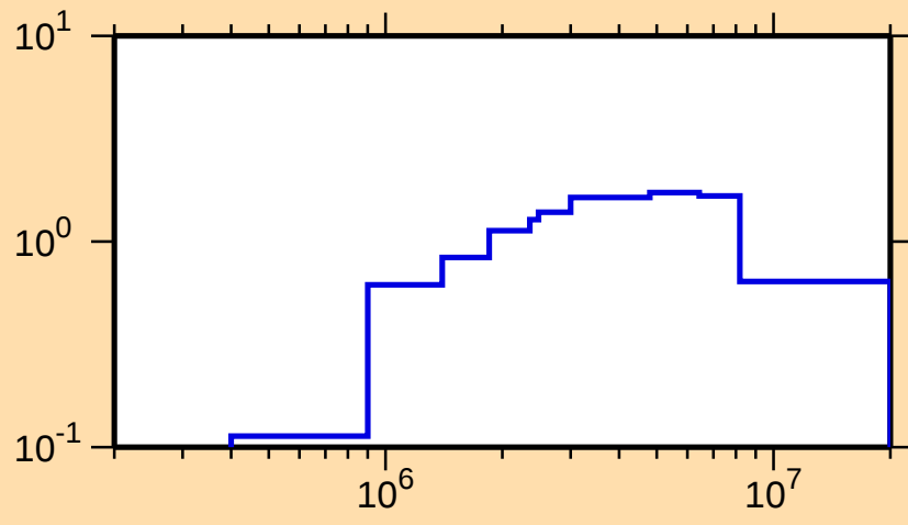
\sigma vs. E for ^{72}\text{Zn}(n,\text{inel.})
