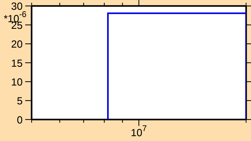
\sigma vs. E for ^{72}\text{Zn}(n,n\alpha)
