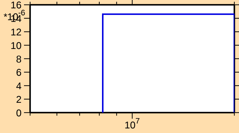
\sigma vs. E for ^{72}\text{Zn}(n,np)
