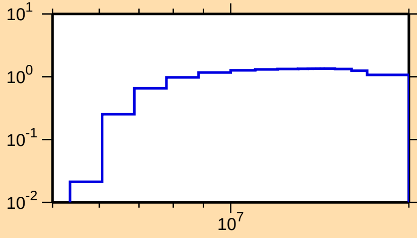
\sigma vs. E for ^{73}\text{Zn}(n,2n)
