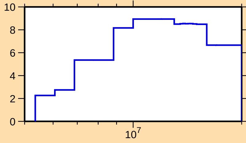
\Delta\sigma/\sigma vs. E for ^{73}\text{Zn}(n,\text{tot.})
