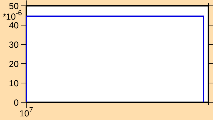
\sigma vs. E for ^{73}\text{Zn}(n,d)
