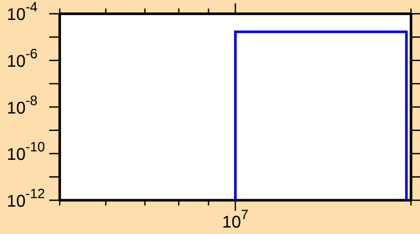
\sigma vs. E for ^{73}\text{Zn}(n,n\alpha)
