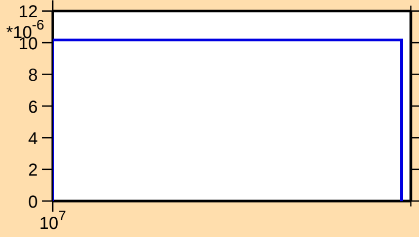
\sigma vs. E for ^{73}\text{Zn}(n,np)
