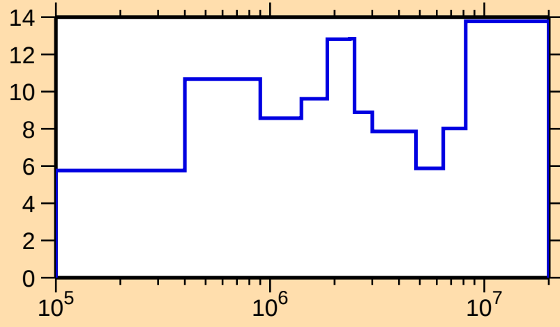
\Delta\sigma/\sigma vs. E for ^{73}\text{Zn}(n,\text{el.})
