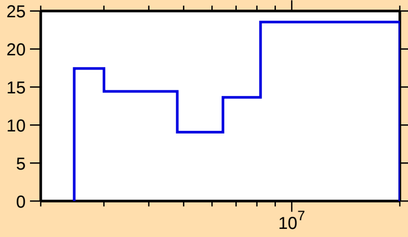
\Delta\sigma/\sigma vs. E for ^{73}\text{Zn}(n,n\text{cont.})
