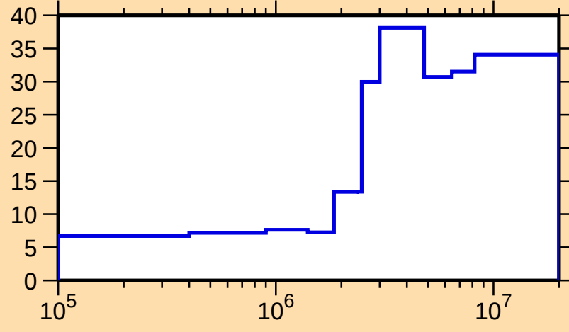
\Delta\sigma/\sigma vs. E for ^{73}\text{Zn}(n,n_1)
