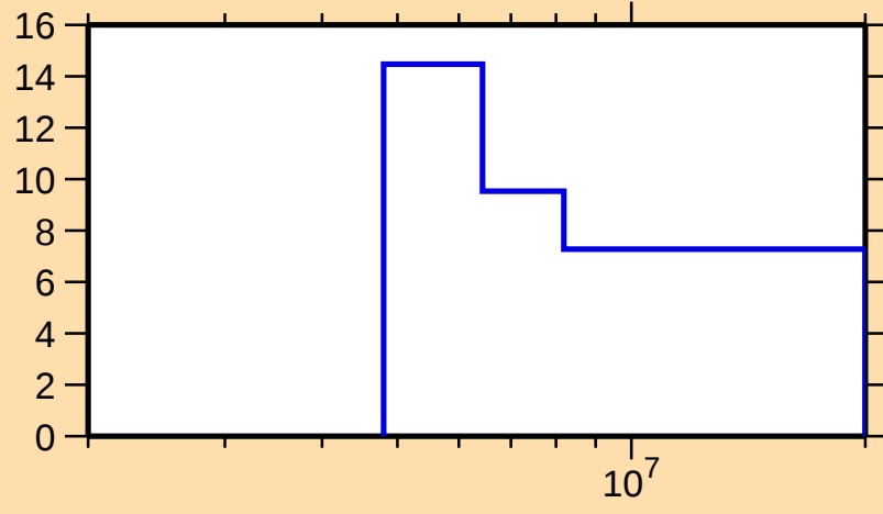
\Delta\sigma/\sigma vs. E for ^{73}\text{Zn}(n,2n)
