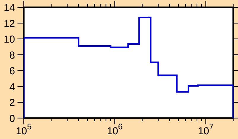
\Delta\sigma/\sigma vs. E for ^{73}\text{Zn}(n,\text{nonel.})
