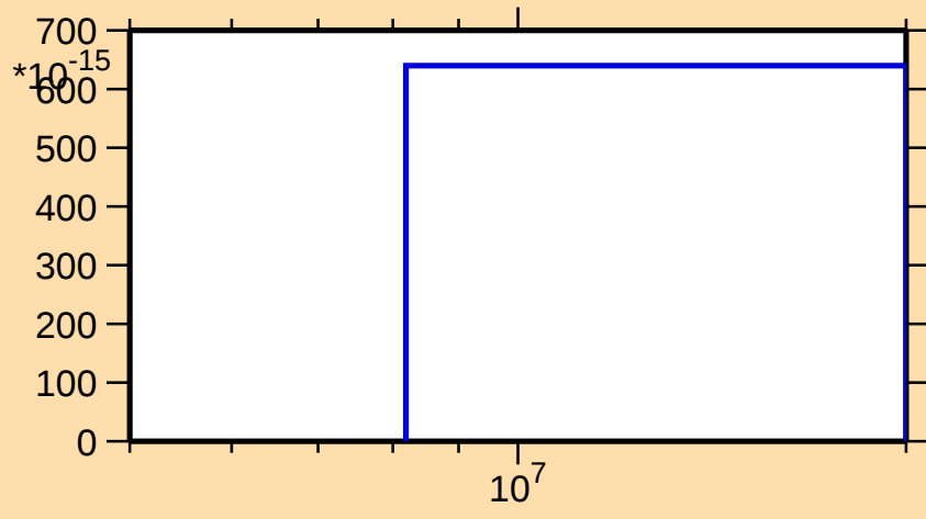
\sigma vs. E for ^{73}\text{Zn}(n,nt)
