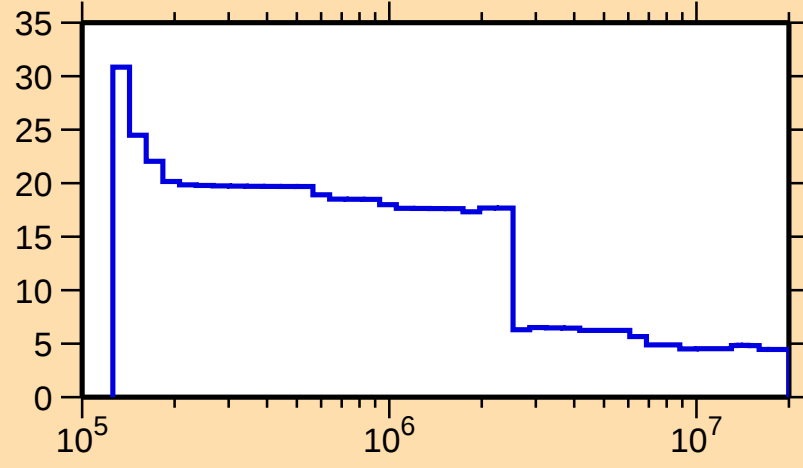
\Delta\sigma/\sigma vs. E for ^{75}\text{Zn}(n,\text{nonel.})
