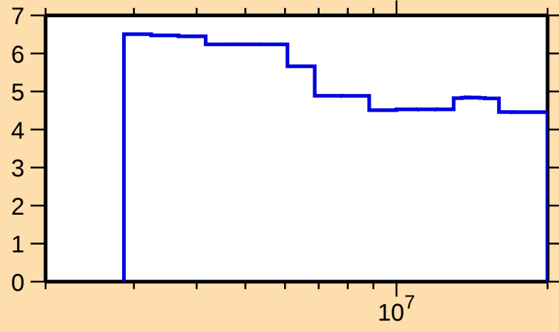
\Delta\sigma/\sigma vs. E for ^{75}\text{Zn}(n,\text{nonel.})
