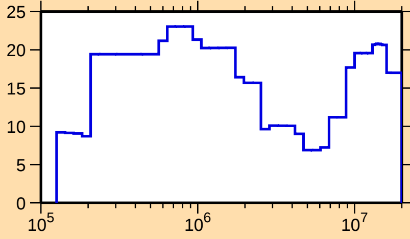
\Delta\sigma/\sigma vs. E for ^{75}\text{Zn}(n,\text{el.})
