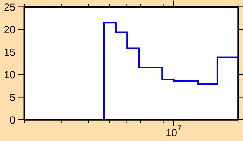
\Delta\sigma/\sigma vs. E for ^{75}\text{Zn}(n,2n)
