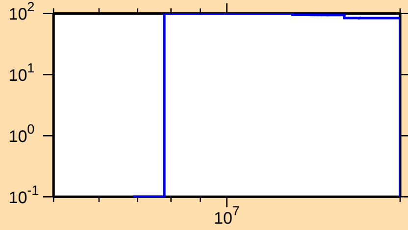
\Delta\sigma/\sigma vs. E for ^{75}\text{Zn}(n,p)
