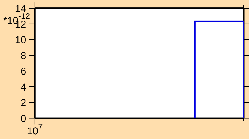
\sigma vs. E for ^{75}\text{Zn}(n,nt)
