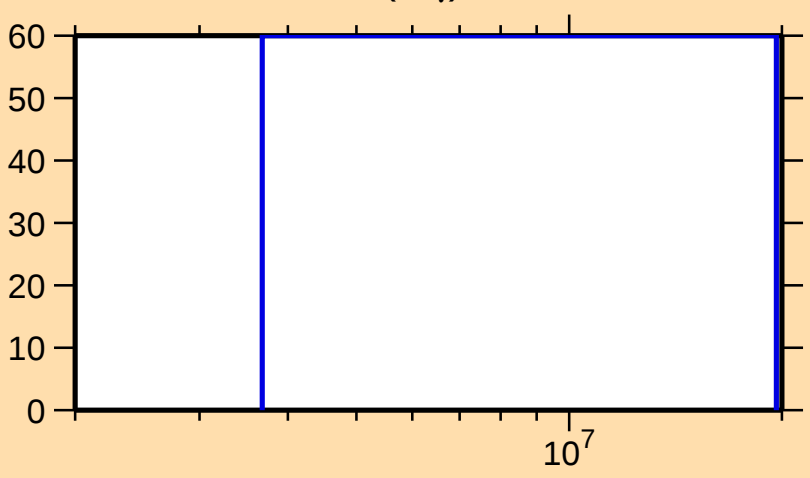
\Delta\sigma/\sigma vs. E for ^{75}\text{Zn}(n,\gamma)
