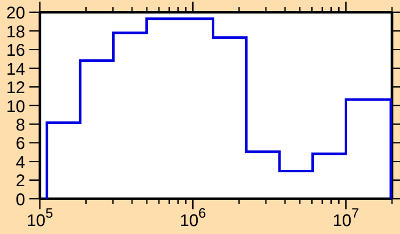
\Delta\sigma/\sigma vs. E for ^{75}\text{Zn}(n,\text{tot.})
