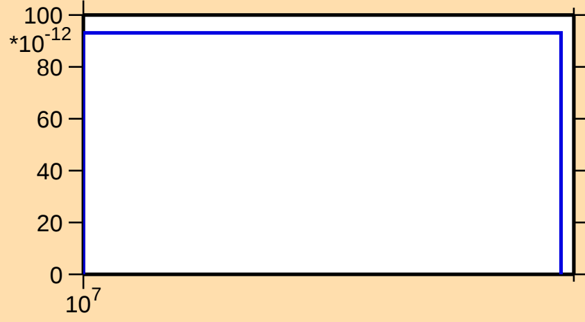
\sigma vs. E for ^{75}\text{Zn}(n,\text{nd})
