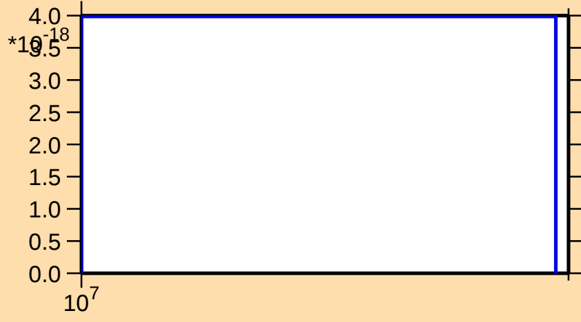
\sigma vs. E for ^{75}\text{Zn}(n,2np)
