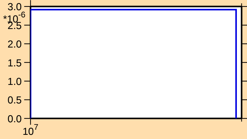
\sigma vs. E for ^{75}\text{Zn}(n,t)
