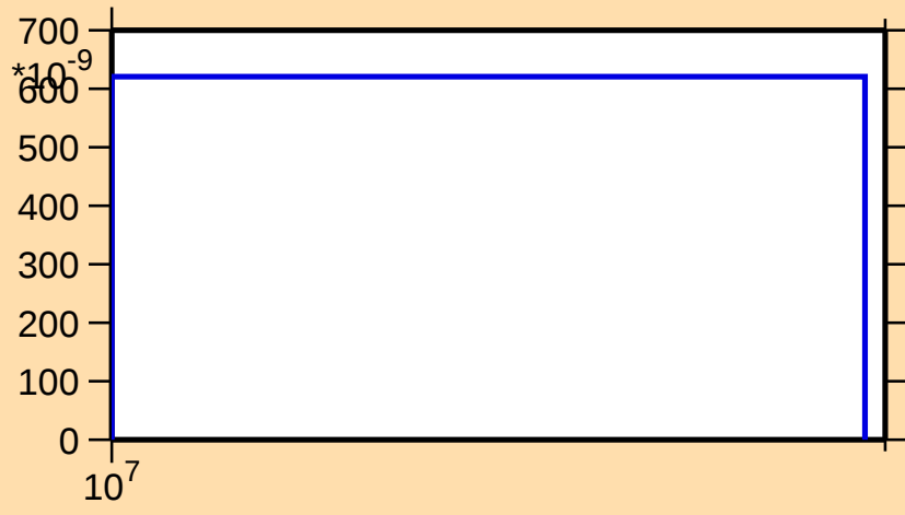
\sigma vs. E for ^{75}\text{Zn}(n,n\alpha)
