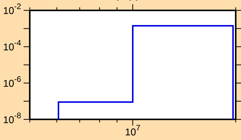
\sigma vs. E for ^{75}\text{Zn}(n,p)
