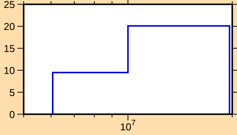
\Delta\sigma/\sigma vs. E for ^{75}\text{Zn}(n,\text{el.})
