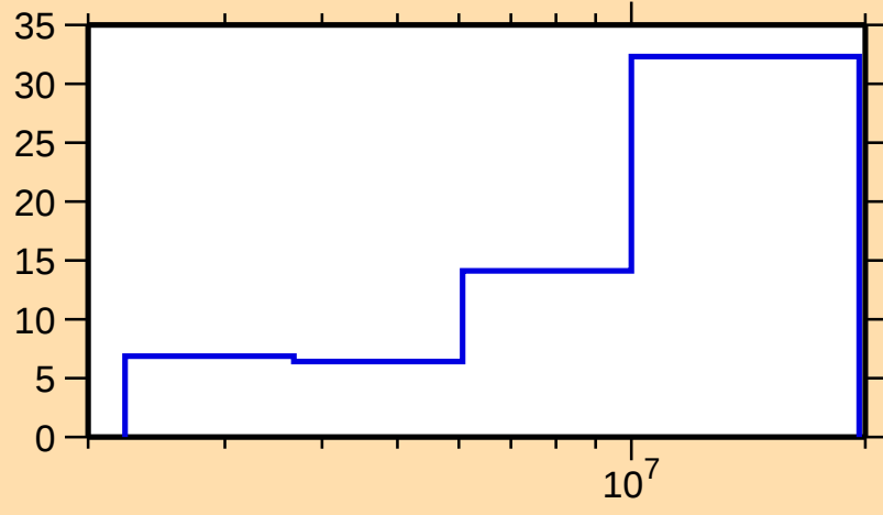
\Delta\sigma/\sigma vs. E for ^{75}\text{Zn}(n,\text{inel.})
