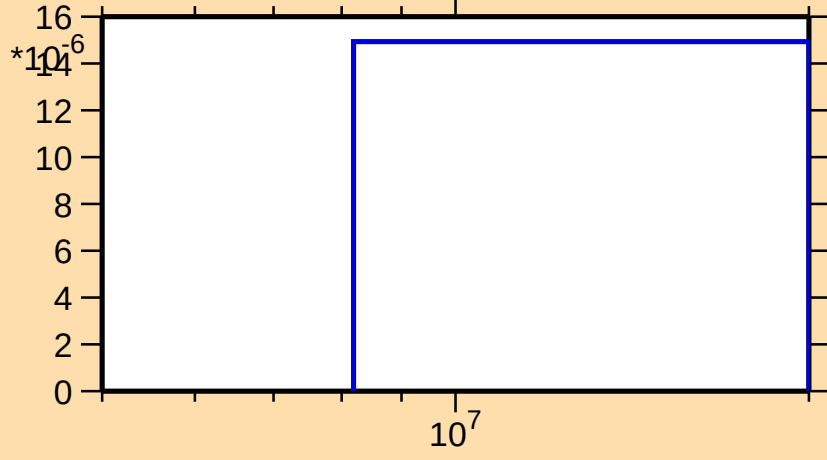
\sigma vs. E for ^{75}\text{Zn}(n,d)
