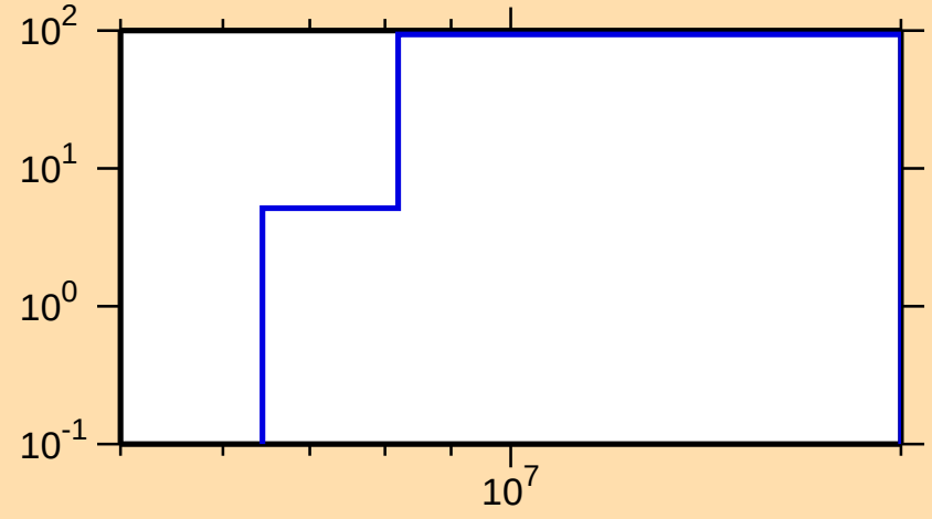
\Delta\sigma/\sigma vs. E for ^{75}\text{Zn}(n,p)
