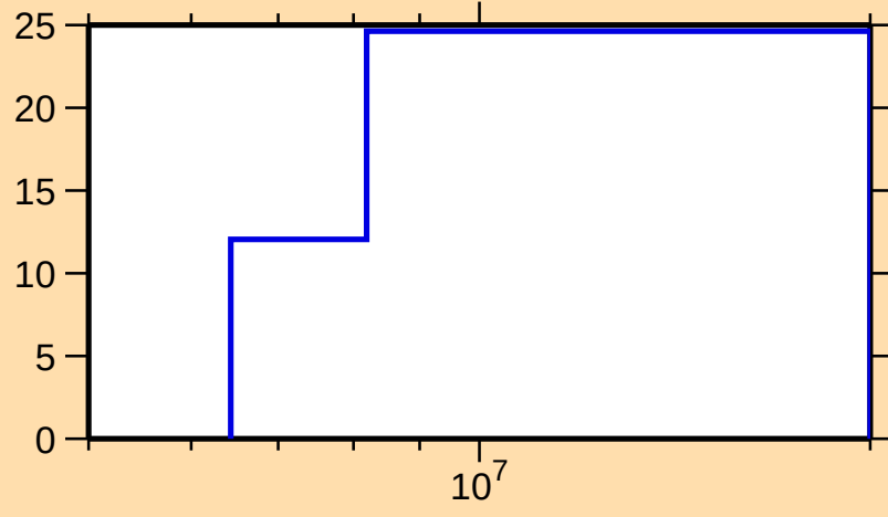
\Delta\sigma/\sigma vs. E for ^{75}\text{Zn}(n,n\text{cont.})
