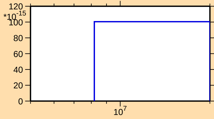
\sigma vs. E for ^{75}\text{Zn}(n,nt)
