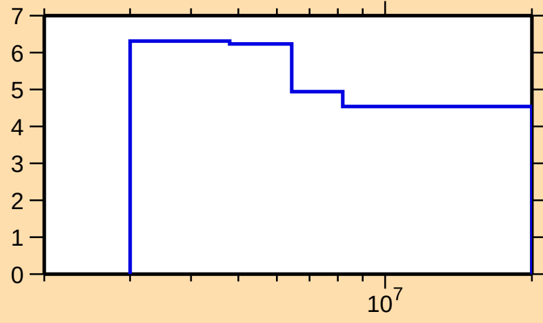
\Delta\sigma/\sigma vs. E for ^{75}\text{Zn}(n,n_{\text{nonel.}})
