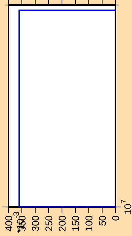
\Delta\sigma/\sigma vs. E for ^{77}\text{Zn}(n,nt)
