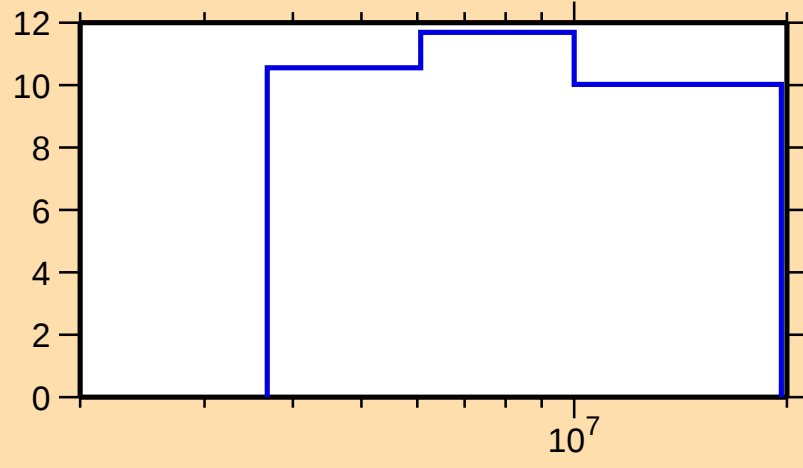
\Delta\sigma/\sigma vs. E for ^{77}\text{Zn}(n,n\text{oncl.})
