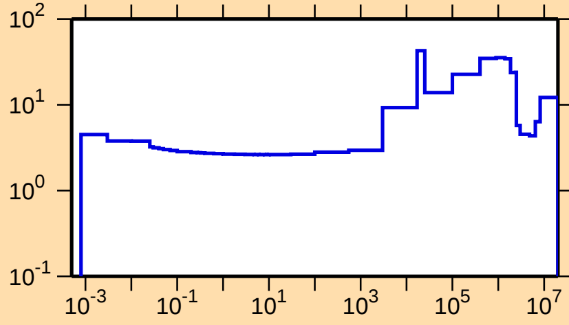
\Delta\sigma/\sigma vs. E for ^{77}\text{Zn}(\text{n,tot.})
