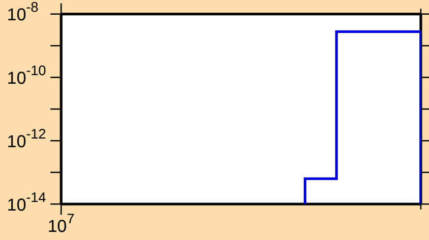
\sigma vs. E for ^{98}\text{Zr}(n,\text{nd})
