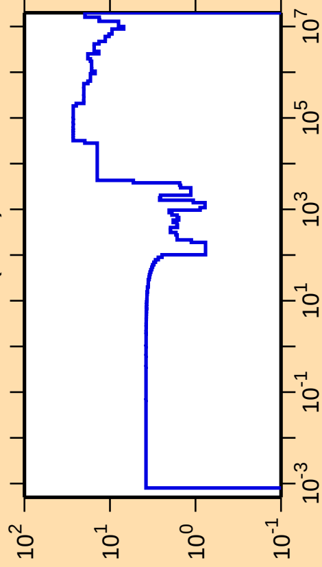
\Delta\sigma/\sigma vs. E for ^{103}\text{Zr}(n,\text{el.})
