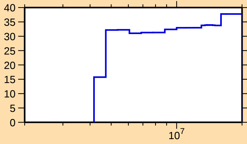
\Delta\sigma/\sigma vs. E for ^{103}\text{Zr}(n,\text{inel.})
