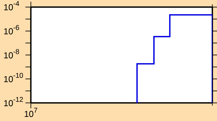
\sigma vs. E for ^{103}\text{Zr}(n,np)
