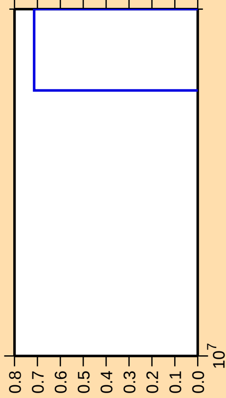
\Delta\sigma/\sigma vs. E for ^{103}\text{Zr}(n,2np)
