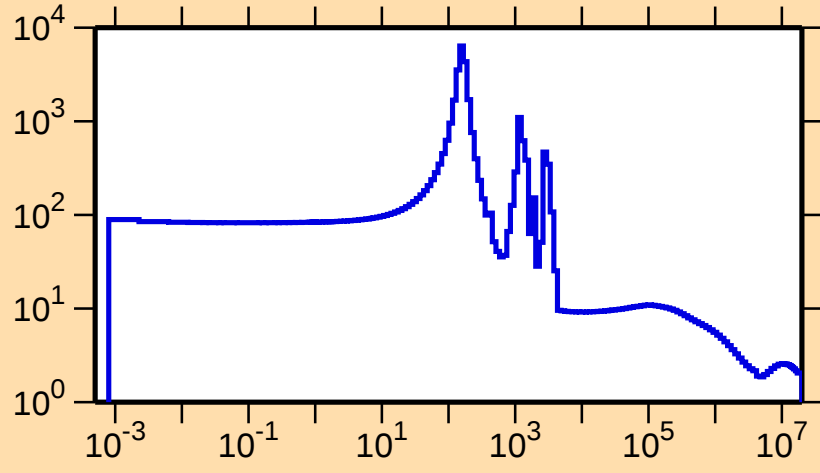
\sigma vs. E for ^{103}\text{Zr}(n,\text{el.})
