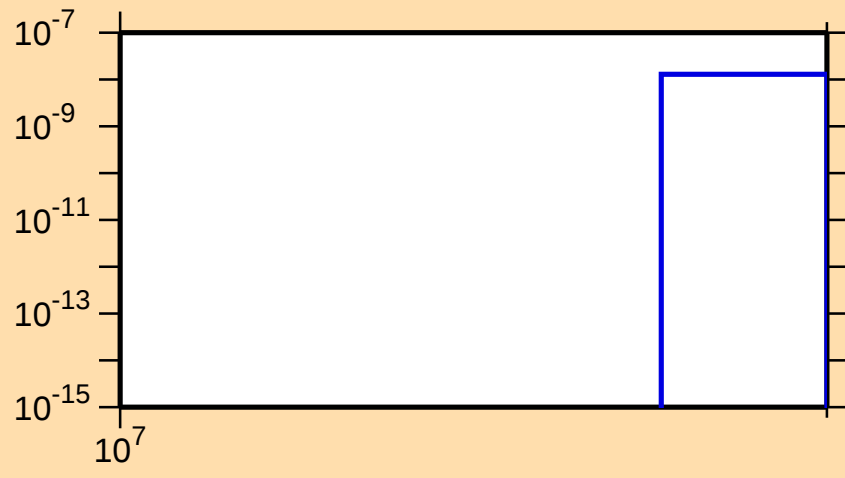
\sigma vs. E for ^{103}\text{Zr}(n,\text{nd})
