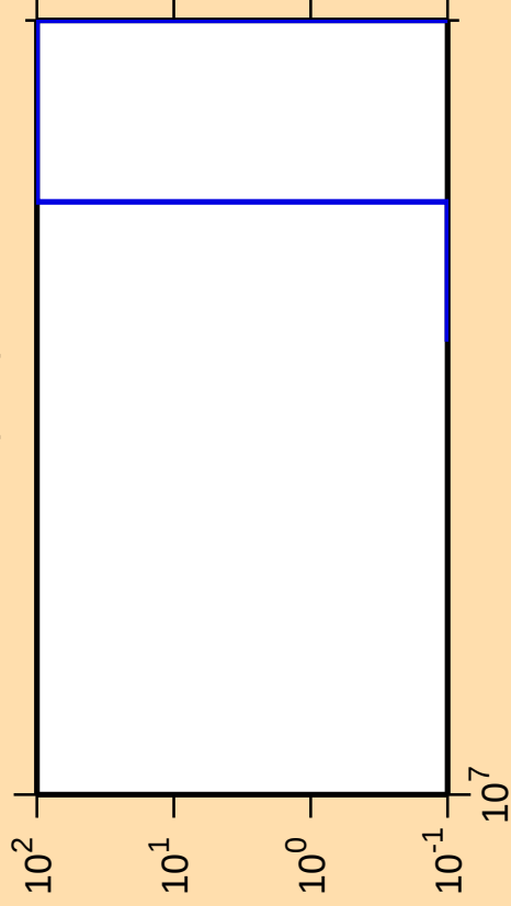
\Delta\sigma/\sigma vs. E for ^{103}\text{Zr}(n,\text{nt})
