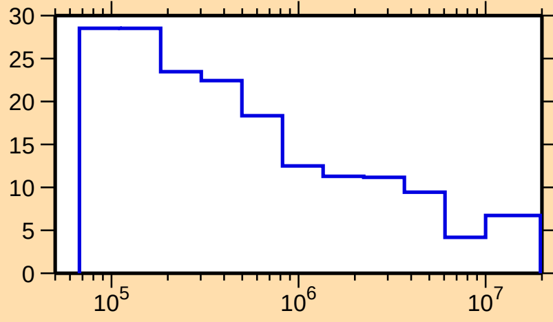
\Delta\sigma/\sigma vs. E for ^{103}\text{Zr}(n,\text{tot.})
