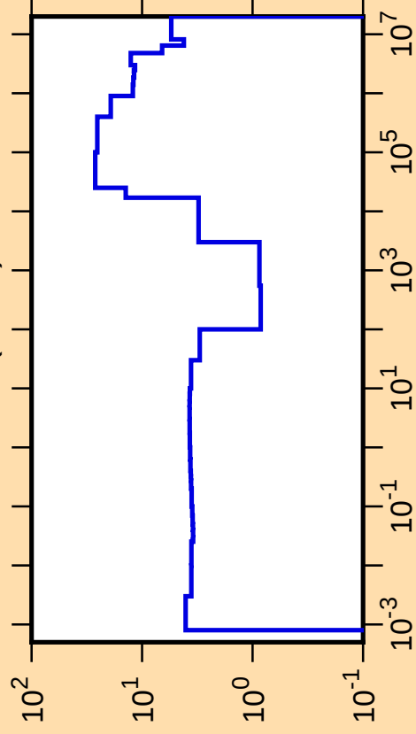
\Delta\sigma/\sigma vs. E for ^{103}\text{Zr}(n,\text{tot.})
