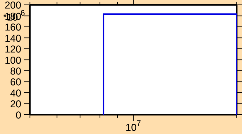
\sigma vs. E for ^{103}\text{Zr}(n,p)
