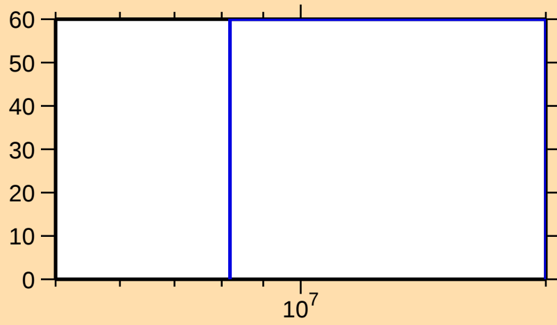
\Delta\sigma/\sigma vs. E for ^{103}\text{Zr}(n,\gamma)
