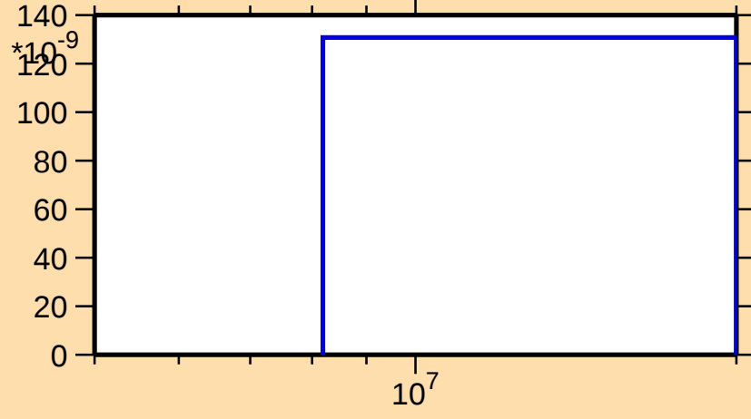
\sigma vs. E for ^{103}\text{Zr}(n,n\alpha)
