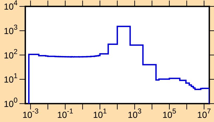
\sigma vs. E for ^{103}\text{Zr}(n,\text{tot.})
