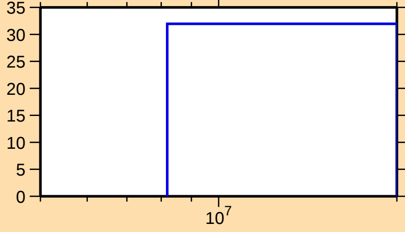
\Delta\sigma/\sigma vs. E for ^{103}\text{Zr}(n,n\text{cont.})
