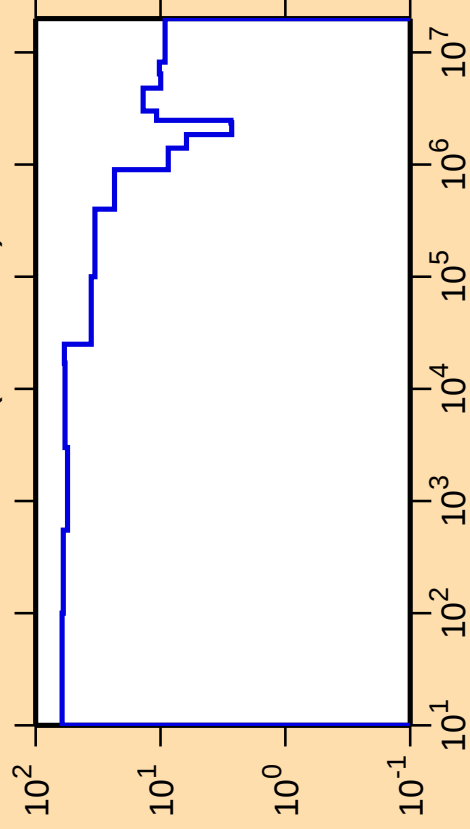
\Delta\sigma/\sigma vs. E for ^{103}\text{Zr}(n,\text{nonel.})
